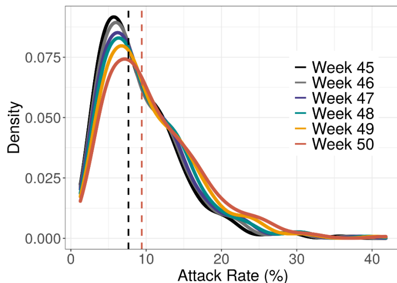
Figure S1: Distribution of attack rates across LTLAs through time. Dashed lines show median AR for week 45 (7.65%, black) and week 50 (9.42%, red) respectively, showing a small increase in naturally acquired immunity through time.
