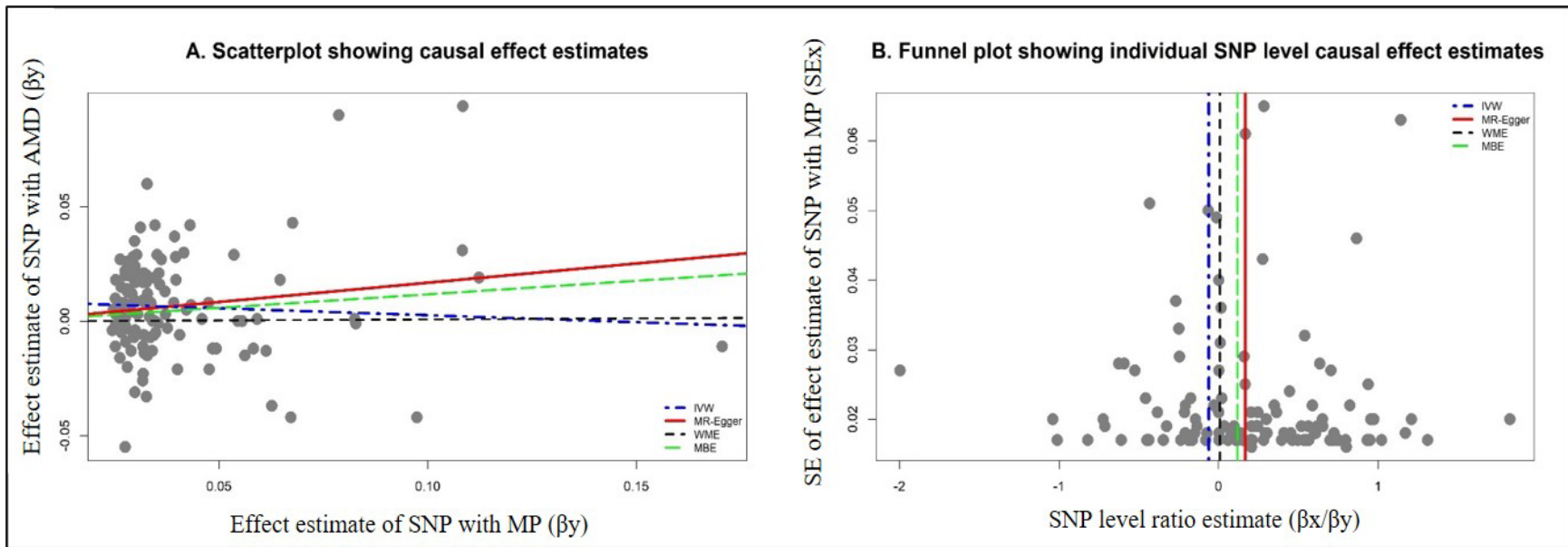
Figure 1. Graphical representation of causal association analysis and assessment of pleiotropy
