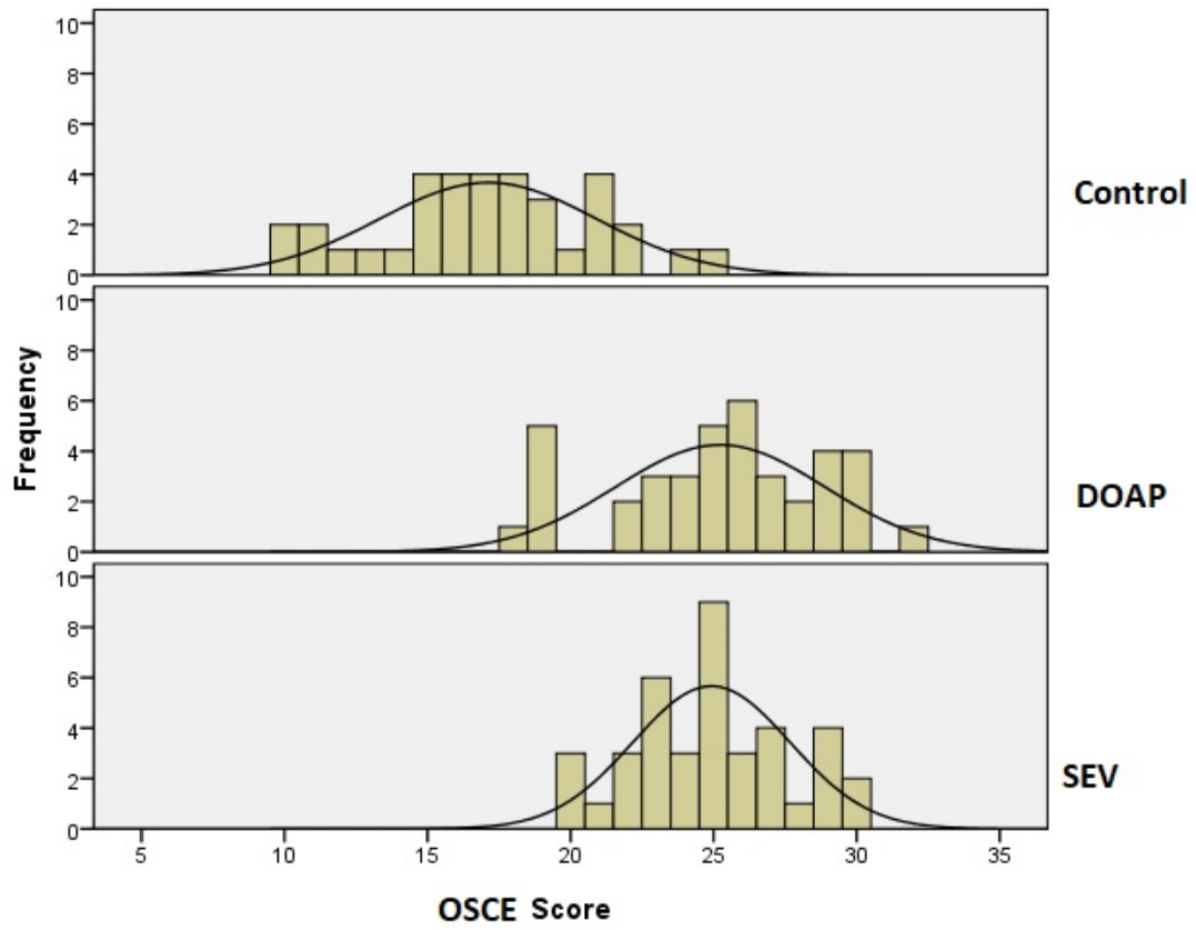
Fig 1: Histogram of OSCE results: Normal Distribution
