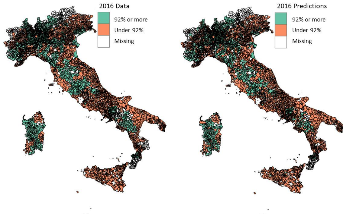
Figure 3. Vaccine Coverage Data (Left panel) and Predictions (Right panel)
