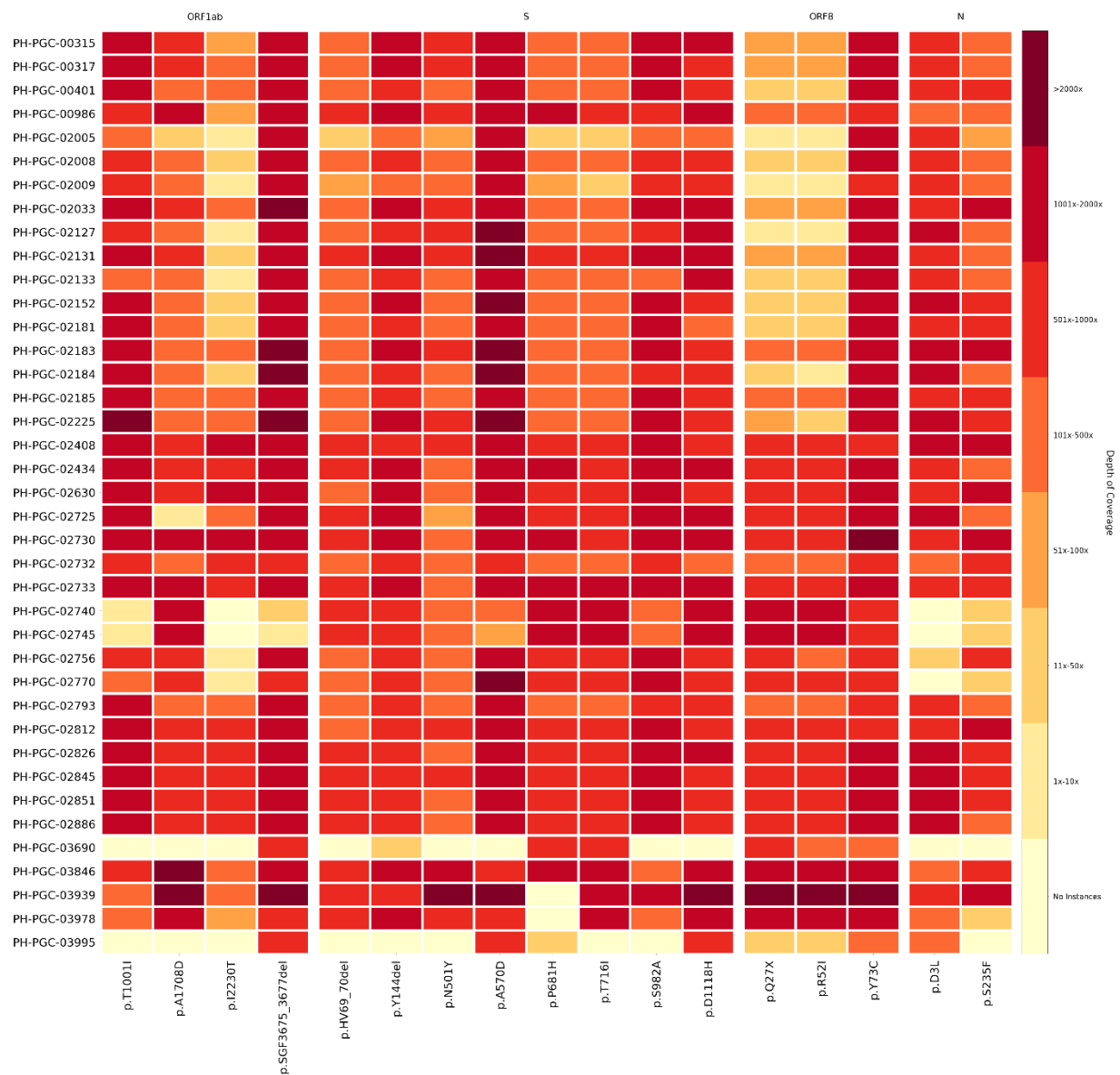
Figure 1. Presence of B.1.1.7 lineage defining mutations in the Philippine SARS-CoV-2 samples. Sequence read coverage for the 17 lineage defining mutations of the B.1.1.7 viruses are shown for each of the locally collected samples classified under the said viral lineage.
