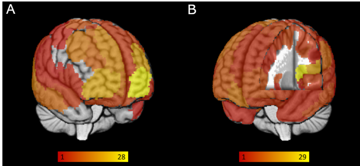
figure S2: Visualisation of node degree changes in Network Based Statistics subnetworks
