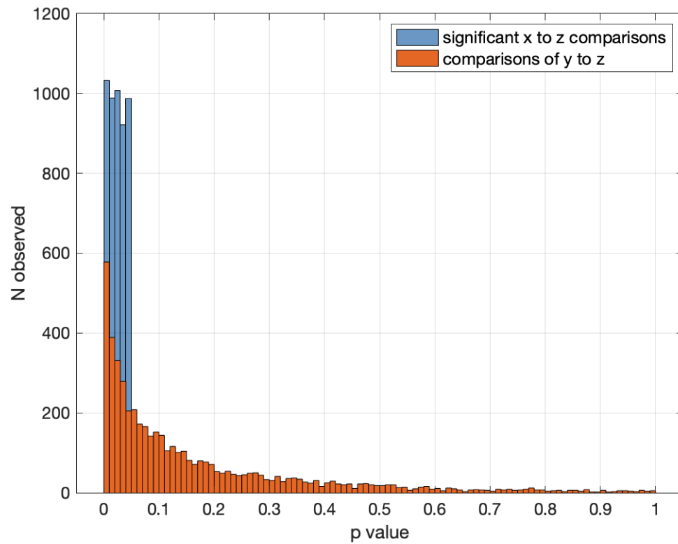
figure S3: Simulation experiment to assess potential statistical bias affecting post-hoc group comparisons
