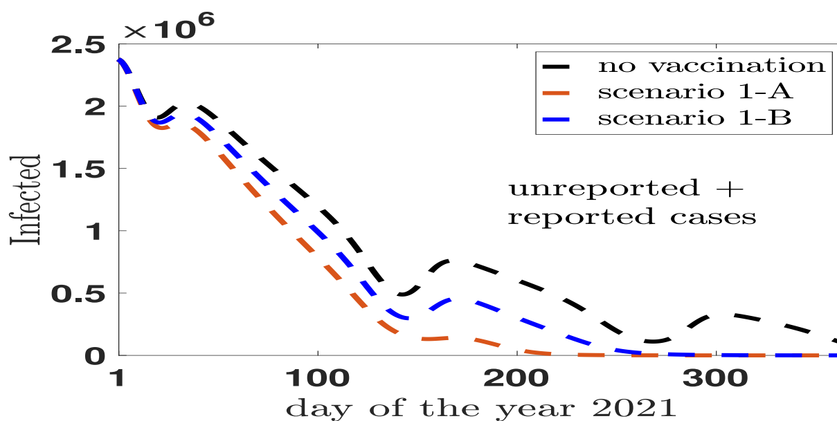
FIG. 14. The reported+unreported cases as a function of the day of the year 2021. The scenario assuming no vaccination (dashed black line) is compared with the scenario 1-A which assumes a constant rate of vaccines of 80000 administrations each day (dashed brown line). The blu (dashed) line (scenario 1-B) shows results for a administration of 40000 vaccines per day at constant rate.
