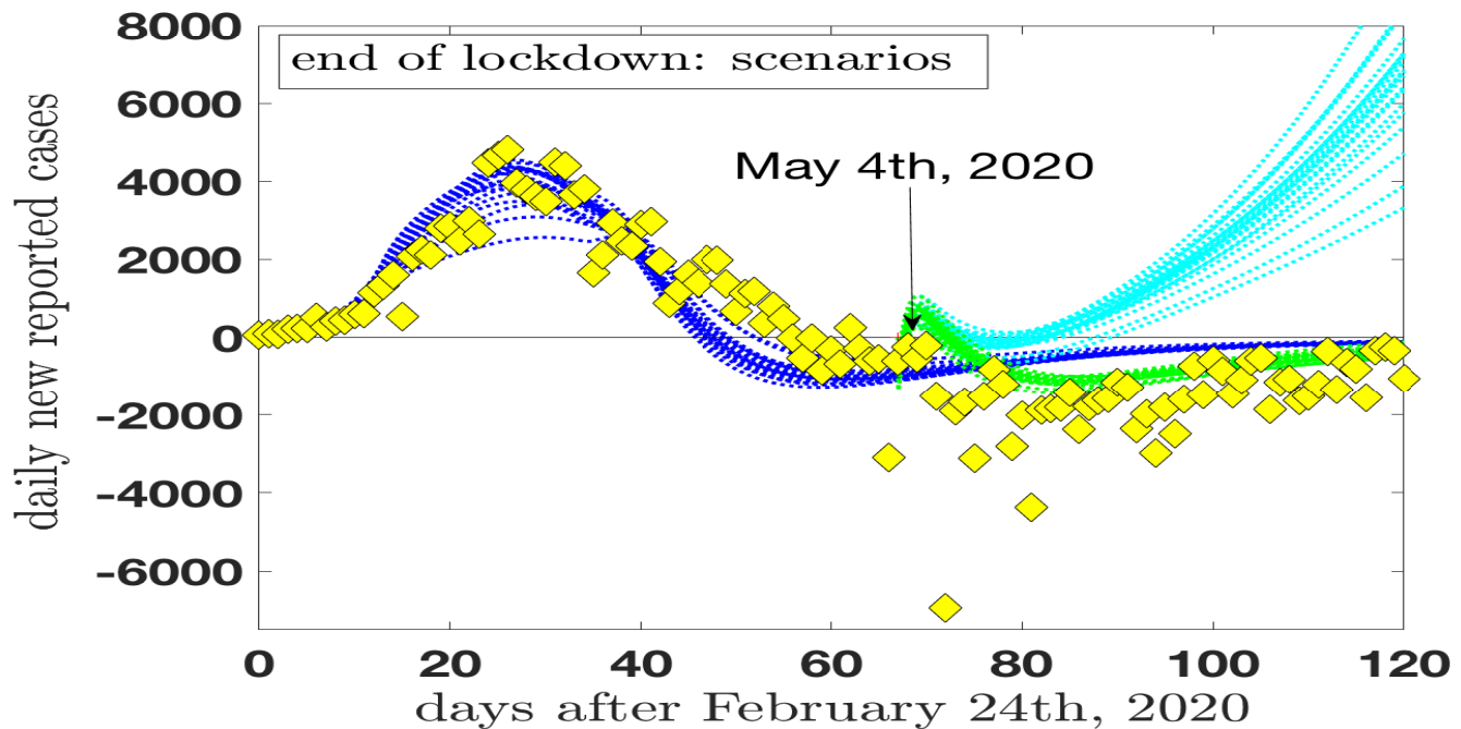
FIG. 5. The model predictions for the daily new reported cases after February 24th, in Italy, are compared with the official data of ref. (Ministero,2020).. In addition to the fully locked scenario (blue lines), two other scenarios are included for a mitigation of the lockdown period in Italy starting from May 4th. Scenario A (cyan lines): a social contact rate somewhat similar to the regular rate (only a reduction of a factor of two is included) would result in a violent secondary outbreak. Scenario B (green lines): A stronger reduction of the contact rate which excludes a large part of social events (school, sports, large events...) with the further inclusion of tracing and quarantine.
