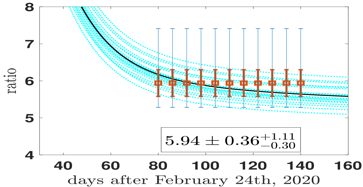
FIG. 9. The ratios of Eqs.(14) and (17), are compared with the cumulative model ratio of Eq.(13) (cyan curves). The smallest error bars take into account the statistical variation suggested by the ISTAT report (ISTAT, 2020). The largest error bars include the modifications induced by the sensitivity and specificity of the IgG and their time-dependence as elaborated by Deeks et al. (Deeks, 2020). See text for discussion.
