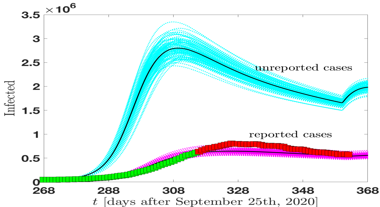
FIG. 11. The MCMC analysis of the infected individuals (reported and unreported cases) in Italy as a function of time in the period September 25th - December 31st. The data for the reported-infected individuals are from (Ministero, 2020) and are compared with our model predictions (magenta curves) which include statistical uncertainties. The reported cases are compared with the predictions for the class of infected non reported cases (asymptomatic and symptomatic) in the same period of time (cyan curves).
