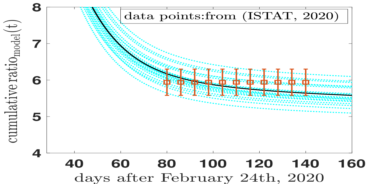
FIG. 7. The fixed ratio of Eq.(14), elaborated from the results of the seroprevalence survey (data-points) is compared with the model ratio of Eq.(13) (cyan curves). See text for discussion.
