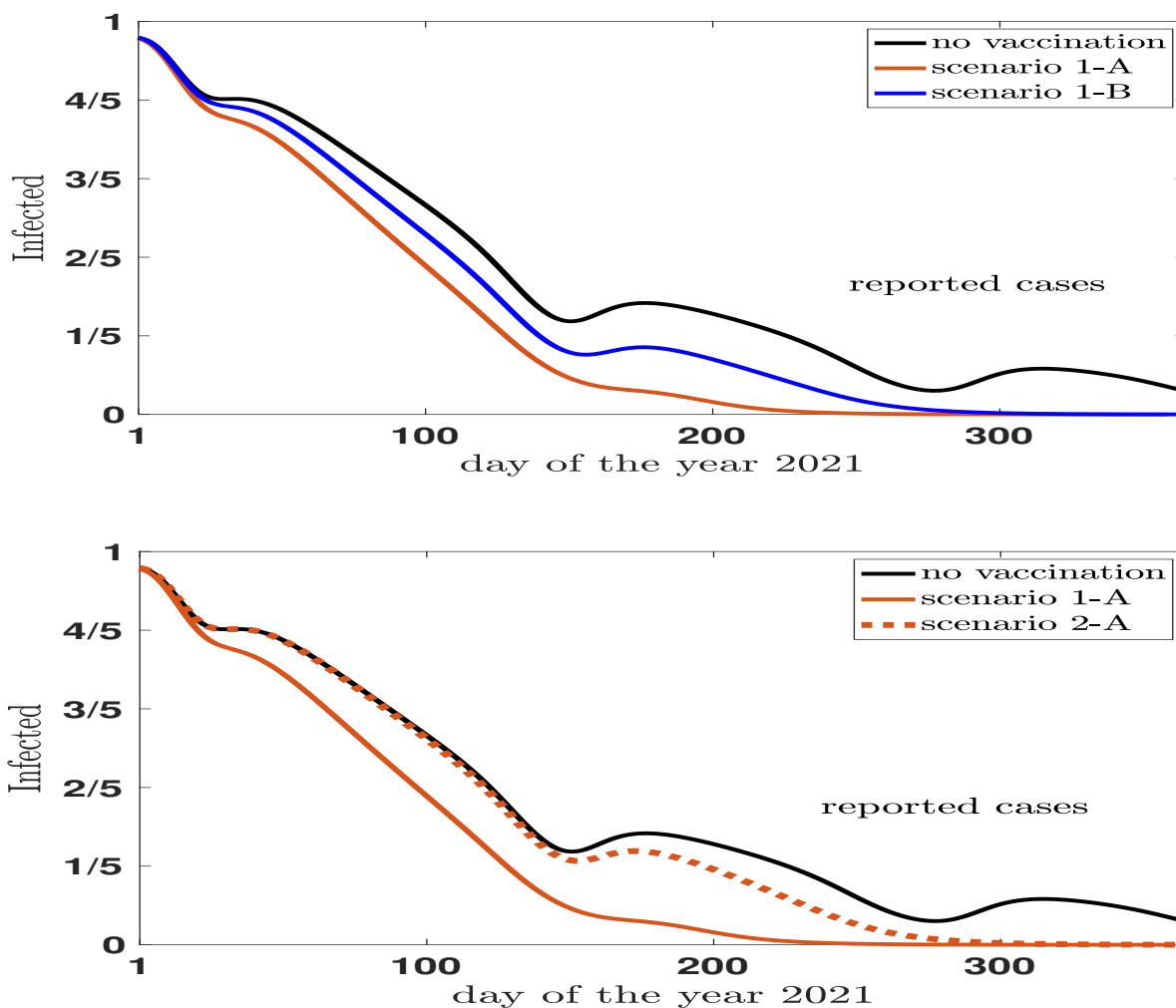
FIG. 13. The fraction of the reported cases as a function of the day of the year 2021. upper panel: The scenario assuming no vaccination (continuous black line) is compared with the scenario 1-A which assumes a constant rate of vaccines of 80000 administrations each day (continuous brown line). The blu line (scenario 1-B) shows results for a administration of 40000 vaccines per day at constant rate. lower pane: The results of a constant rate of vaccine administration (80000 per day, continuous brown line) is compared with the results of no vaccination (black line) and the scenario 2-A where the rate is not constant and a low starting period is compensated by an accelerated second administration period (see Fig. 12).
