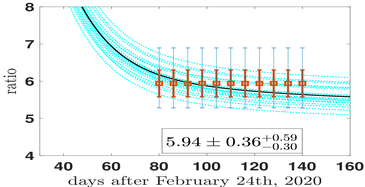
FIG. 8. The ratios of Eqs.(14) and (15), are compared with the cumulative model ratio of Eq.(13) (cyan curves). The smallest error bars take into account the statistical variation suggested by the ISTAT report (ISTAT, 2020). The largest error bars include the modifications induced by the sensitivity and specificity of the IgG tests as indicated by the same ISTAT report. See text for discussion.
