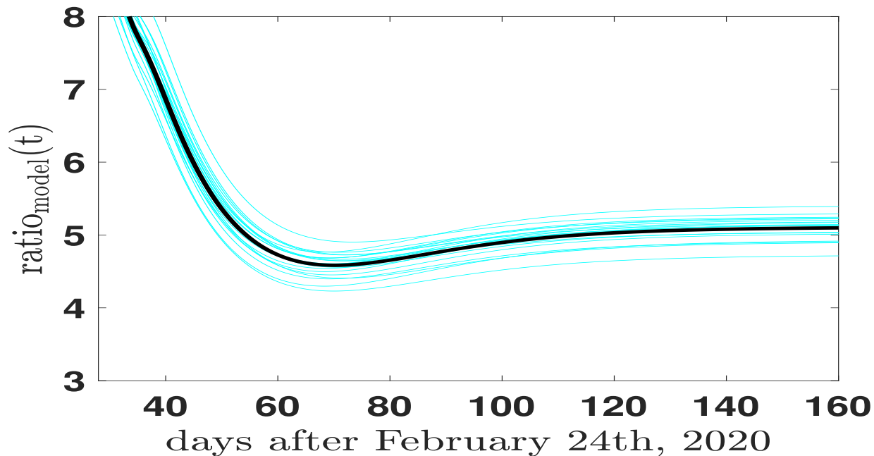
FIG. 6. The model ratio of Eq.(12) as a function of time
