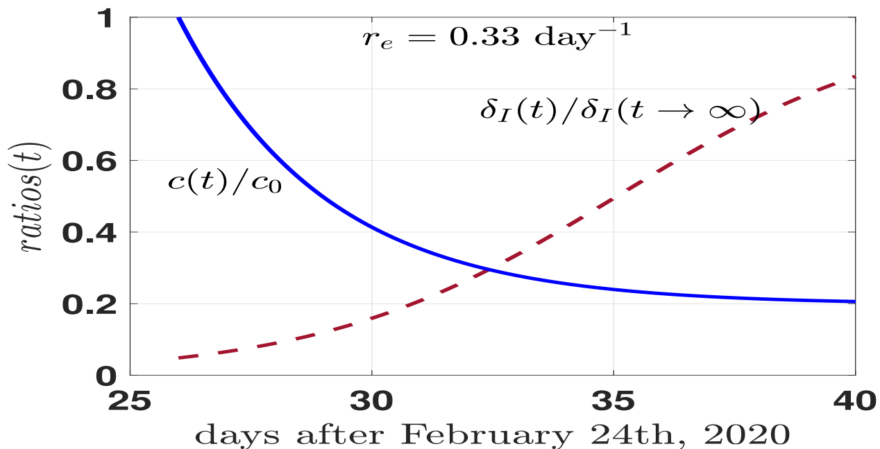
FIG. 3. Modelling the variation in time of the contact rate per person c(t) ( c(t=0) = c_0 ) and of the rate from infected to quarantined classes \delta_I(t) (cfr. Eqs.(9),(10)).
