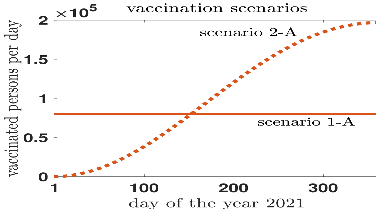
FIG. 12. A constant number of person are vaccinated per day during the year 2021: 80000, full curve (scenario 1-A). Alternatively in scenario 2-A an increasing number of people are vaccinated during 2021 allowing for a less strong starting effort. The total number of vaccinated people result (almost) 30 million for both scenarios, at the end of the year.
