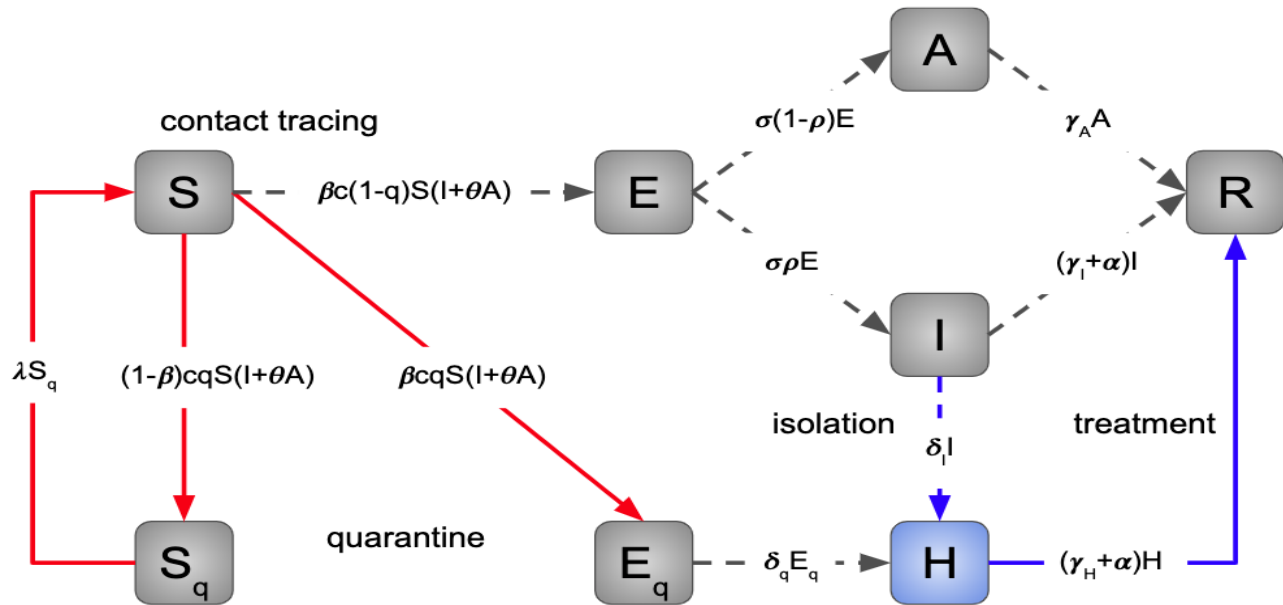
FIG. 1. Diagram of the model simulating the novel Coronavirus (Sars-CoV-2) infection in Italy. The population is stratified in Susceptible ( S ), exposed ( E ), asymptomatic infected individuals ( A ), infected with symptoms ( I ), detected infected (hospitalized in a large sense) ( H ) and recovered ( R ), quarantined susceptible ( S_q ), isolated exposed ( E_q ) compartments. Interventions like intensive contact tracing followed by quarantine and isolation are indicated (Tang, 2020. Inf. Dis. Model.).
