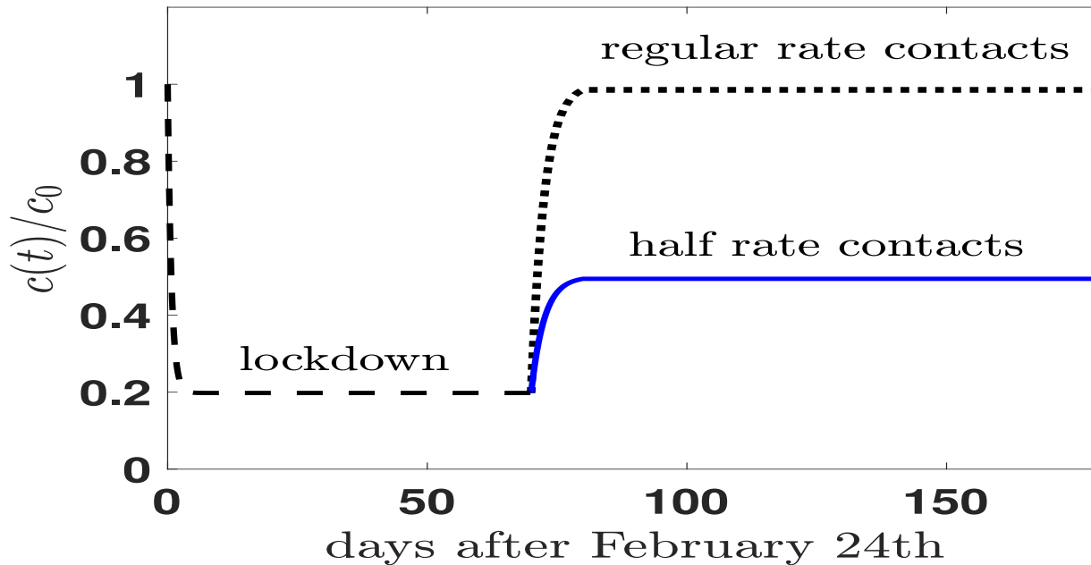
FIG. 4. Time behavior of the contact rate simulating a possible secondary event in Italy at day=70, after February 24th, when the stringent measures of isolation are hypothetically relaxed. Two scenarios are introduced, the scenario of a rapid return to the old style of life (regular rate contacts), and a more realistic scenario where only half of the regular contacts are activated.
