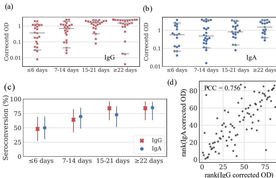
Figure 3: Dynamics of ST protein-specific IgG and IgA response. (a-b) Corrected OD values of COVID-19 positive samples collected at different time points post-onset of symptoms (n=25 for each time interval). Value for each sample is represented by a point on the scatter plot. Median, 5th percentile and 95th percentile values are shown by horizontal gray lines. (c) Percentage seroconversion of patients based on IgG and IgA response to ST protein ELISA as a function of time. Vertical lines show 95% confidence intervals (d) Comparison between ranks of the IgG and IgA corrected OD values.
