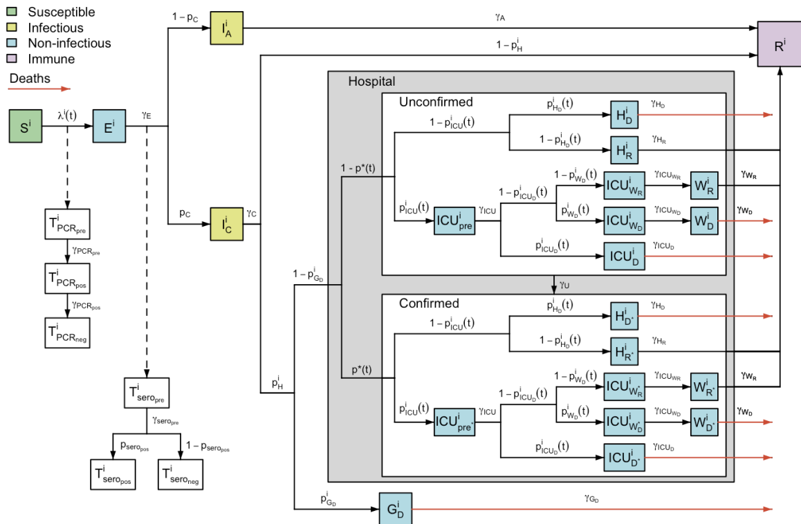
203 204 Figure S 2: Model structure flow diagram with rates of transition between infection states. Variable 205 names defined in text.
