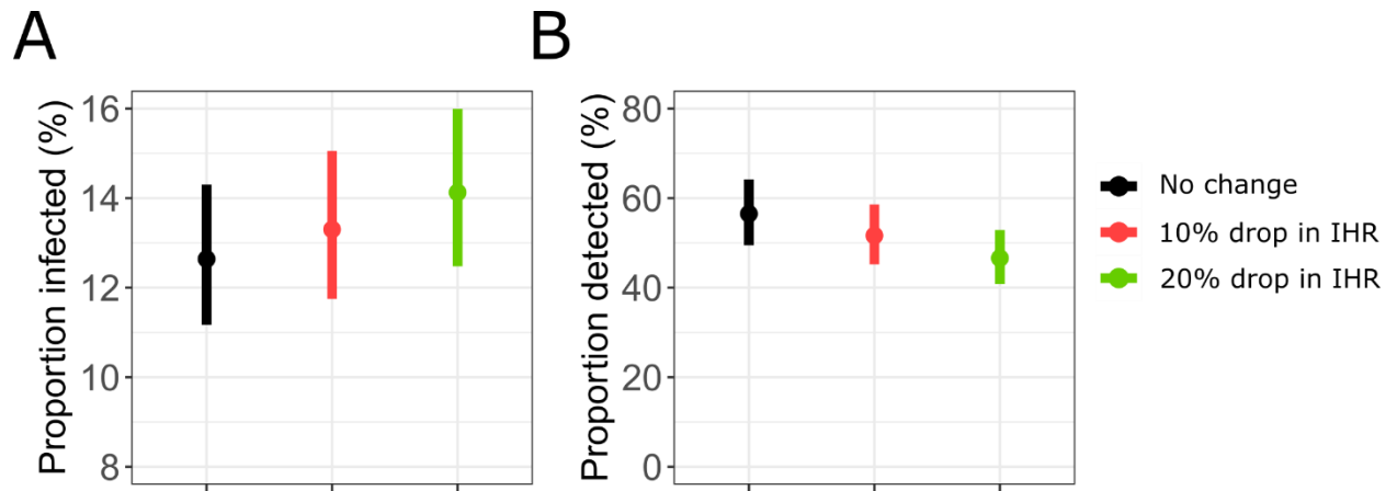
Figure S2. Impact of a reduction in IHR during the second wave on the proportion of infected (A) and the proportion of cases detected by surveillance (B).
