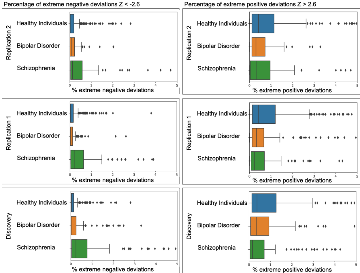
Supplementary Figure 2: Percentage extreme deviations at |Z|=2.6 per participants plotted as boxplot for each group. The results replicate well across samples. In the lower panel we depict results based on the data reported in Wolfers et al. 2018, Jama Psychiatry .
