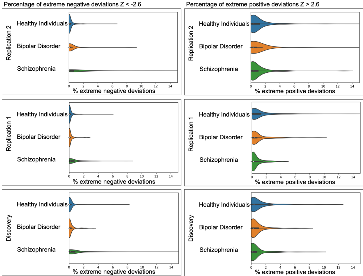
Supplementary Figure 3: Percentage extreme deviations at |Z|=2.6 per participants plotted as violin-plot for each group. The results replicate well across samples. In the lower panel we depict results based on the data reported in Wolfers et al. 2018, Jama Psychiatry .
