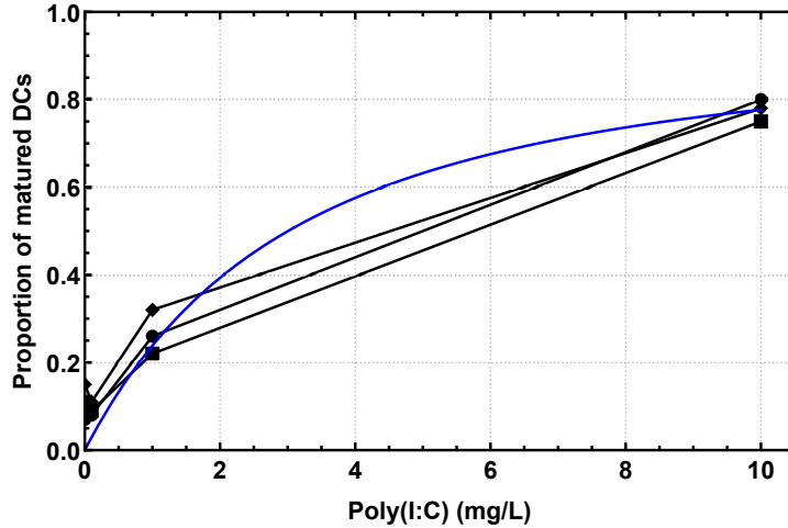
Figure 1. Estimation of parameters r_D and K_a . Blue line represents the function: f(x) = 1 - \exp\left(-\frac{r_D x}{K_a + x}\right) , with r_D = 3 and K_a = 10 , fitted to data extracted from Figure 6A in [5].
