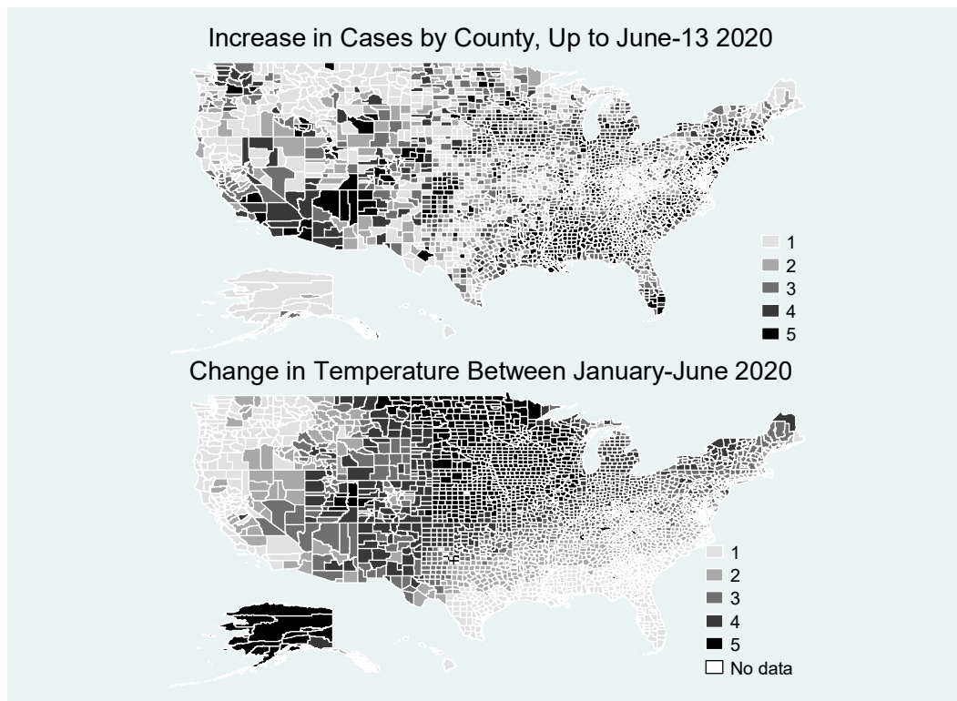
Figure 1 – Changes in Temperature and Confirmed Cases between 22-January and 13-June 2020 Across US Counties
