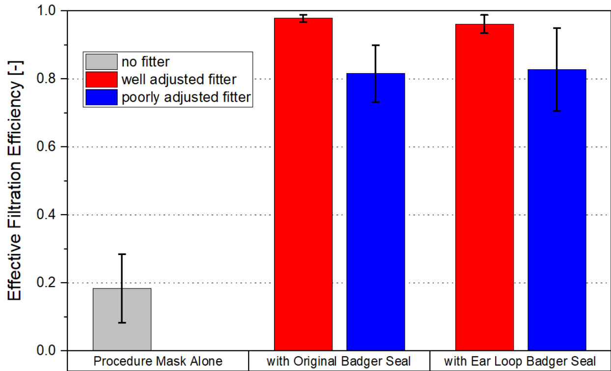
Figure 1: Fit test results with the procedure mask alone and with the Badger Seal Mask fitter both well adjusted and poorly adjusted.
