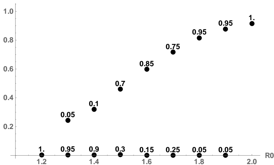
Fig. 3. The means of the large and small values and the probability with which each case occurs. (n0 = 10000, number of runs per R0 = 20, initial immunity rate = 0)
