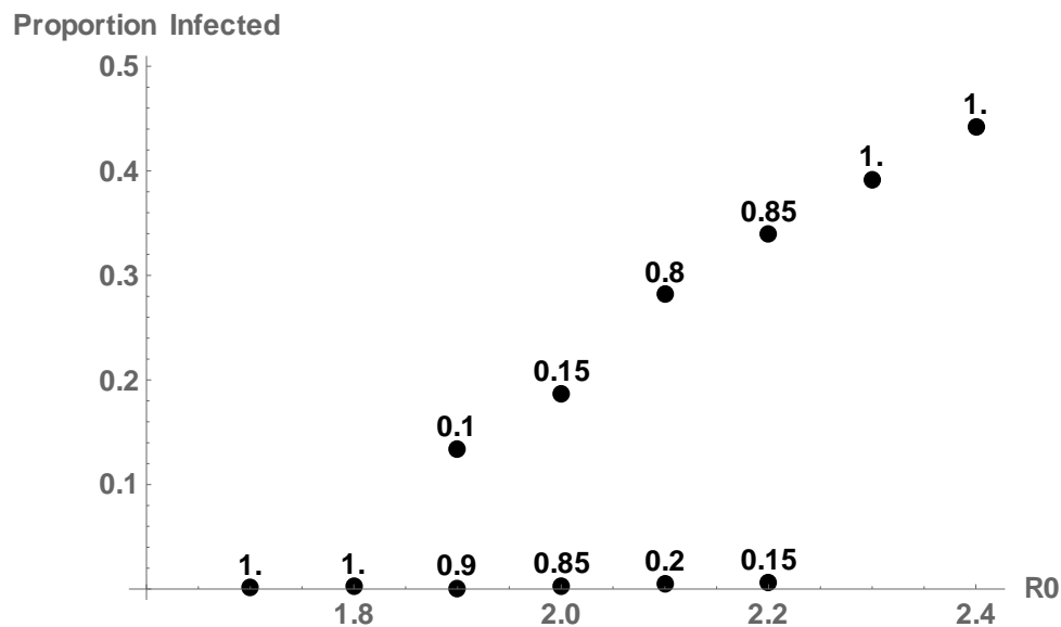
Fig. 5. The means of the large and small values and the probability with which each case occurs. ( n_0 = 10000 , number of runs per R_0 = 20 , initial immunity rate = 0.3)
