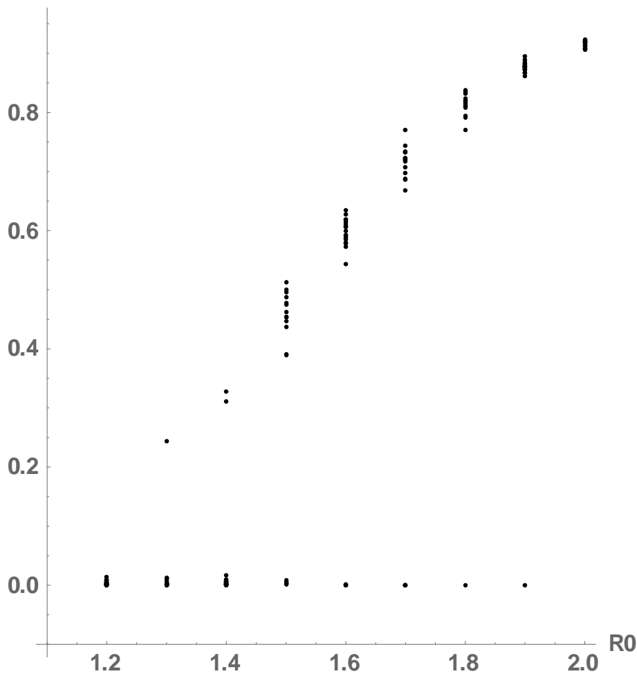
Fig. 2. Results for the number of infected individuals for various R0 values. For each R0, 20 points are plotted, some of which are very close to one another. To make the graph easier to read, the y-axis was shifted by -0.1.
