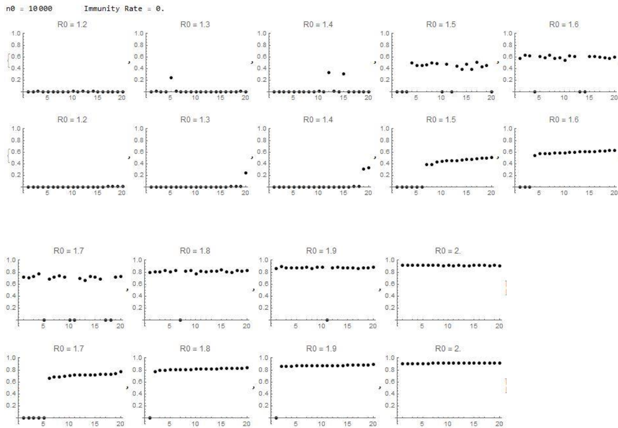
Fig. 1. Results for the number of infected individuals for 20 runs with different R_0 values. The top row shows the proportion of infected individuals in each run of the simulation, the bottom row the same values, ordered by size.
