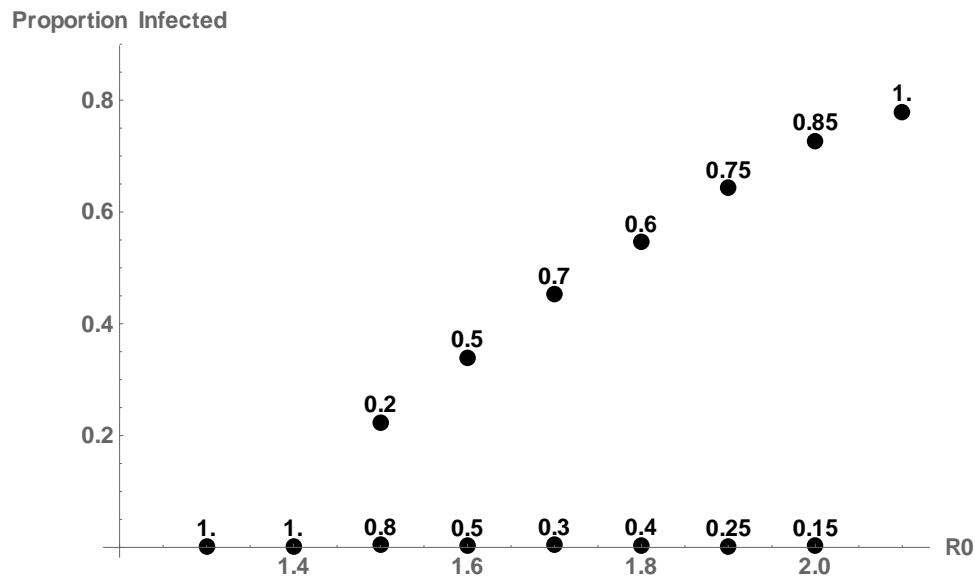
Fig. 4. The means of the large and small values and the probability with which each case occurs. ( n_0 = 10000 , number of runs per R_0 = 20 , initial immunity rate = 0.1)
