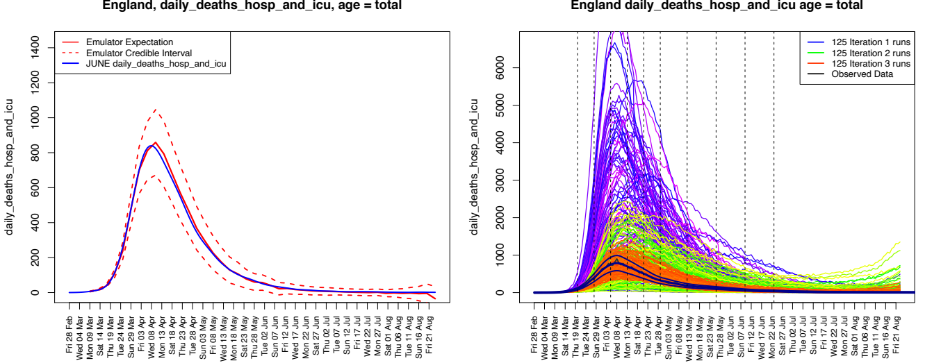
Figure 27: Left Panel: an example diagnostic showing the emulator prediction E_D(f_i(x)) for f_i(x) across several time points (the solid red line) and the prediction interval E_D(f_i(x)) \pm 3\sqrt{\text{Var}_D(f_i(x))} (the red dashed lines) along with the held out smoothed run output f(x) (the blue line). The emulator captures the behaviour of the JUNE model well. Right panel: daily hospital deaths for all of England, showing the progression of the runs from iterations 1, 2 and 3 used in the history matching process (in purple, green and red respectively). Observed data (smoothed and original) in black. Vertical dashed lines: emulated outputs.
