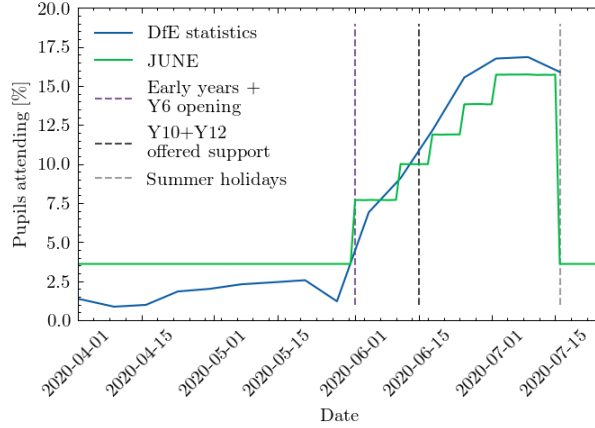
Figure 16: School attendance in JUNE compared to data collected by the UK’s Department for Education [66]
