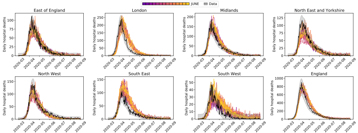
Figure 18: Daily hospital deaths for each region in England, and England itself, for a number of realisations of JUNE as described in this section. Observed data in black with 3 standard deviation error bands. Data from CPNS [71].
