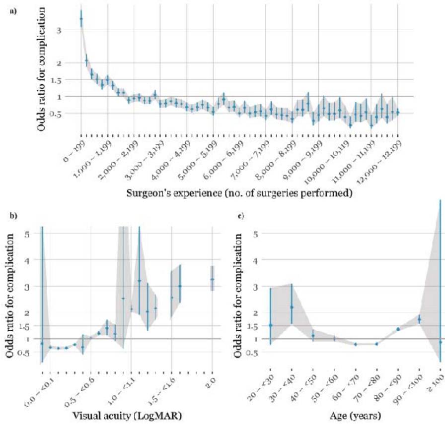
Figure 1. a) Odds ratio for complication as a function of the surgeon's experience expressed as the number of surgeries performed, in intervals of 200. b) Odds ratio for complication as a function of BCVA in LogMAR, in intervals of 0.10. Empty areas in the graph indicate missing data due to an artefact after conversion from Snellen scores to LogMAR values. c) Odds ratio for complication as a function of patient age in years, in intervals of 10 years.
