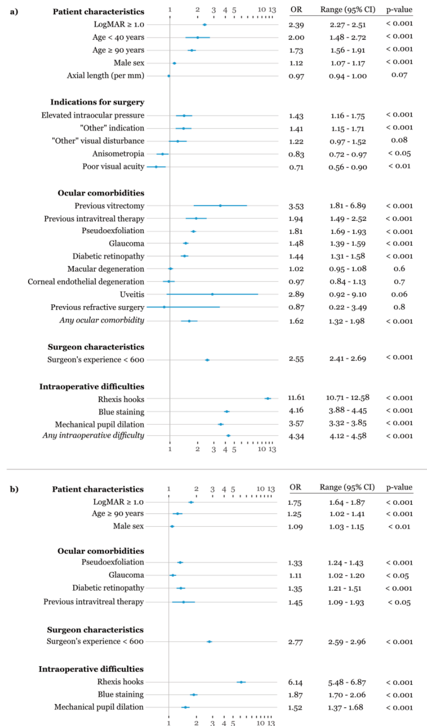
Figure 2. a) Unadjusted odds ratios of risk factors. Variables that cross the vertical line at a value of 1 are nonsignificant. Error bars indicate 95% confidence interval (95% CI). b) Adjusted odds ratios of risk factors in multivariate logistic regression model. Variables that cross the vertical line at 1 on the x-axis indicate nonsignificance. Error bars indicate 95% confidence interval. OR = odds ratio; 95% CI = 95% confidence interval.
