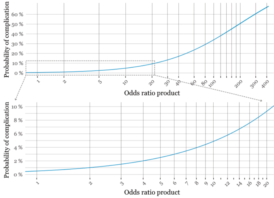
Figure 3. Probability (or risk) of complication as a function of the odds ratio product. The probability of complication can be read off the y-axis after calculating the product of the odds ratios.
