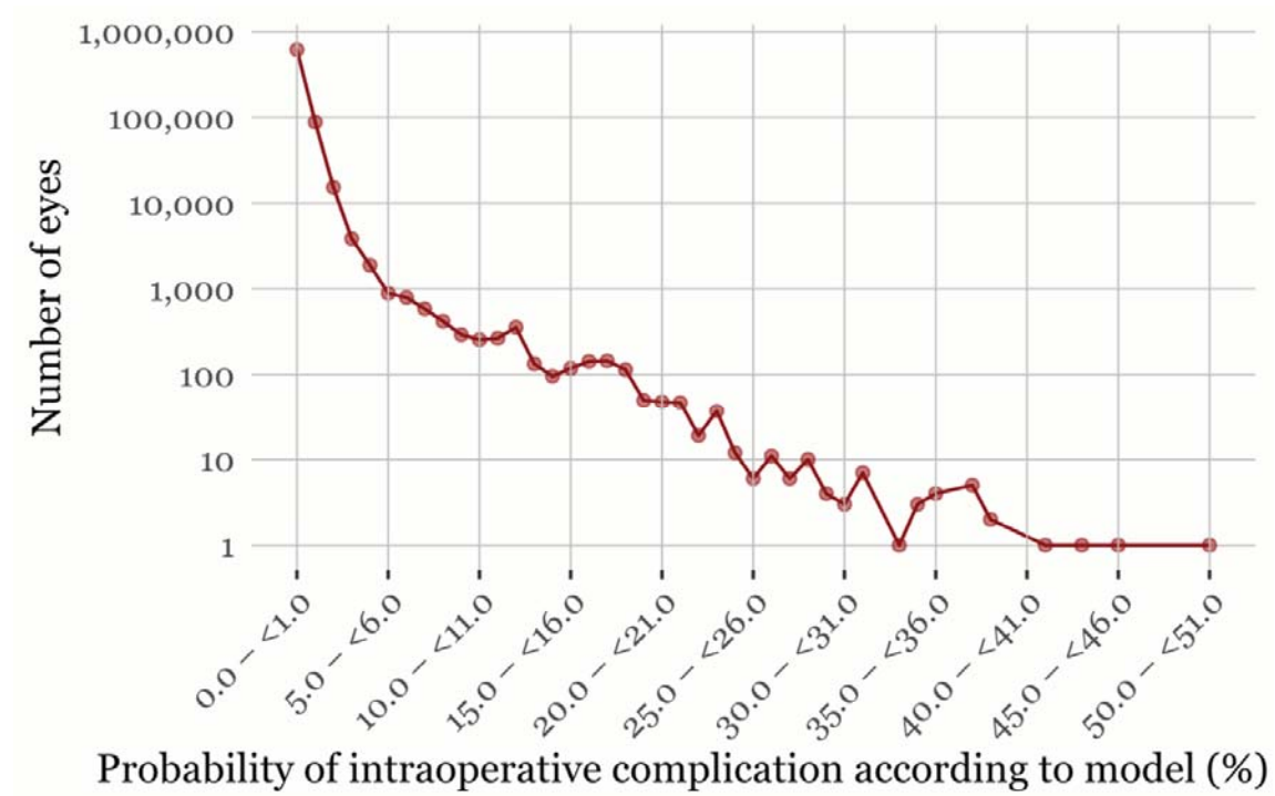
Figure 4. Frequency of the probability of intraoperative complication of the eyes in the dataset (note logarithmic y-scale). The risk of complications was low for most eyes.
