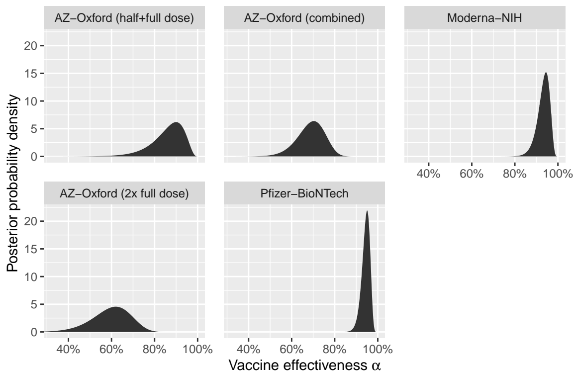
Figure 1: Posterior distributions
