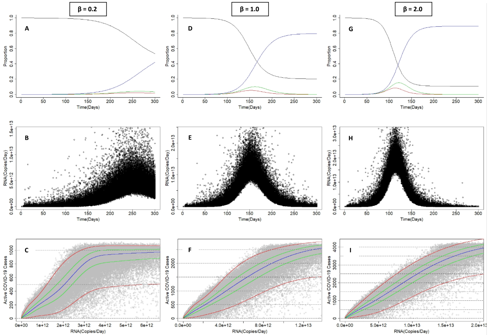
Figure S1: SEIR model for three \beta values. Panels A, D, G: Proportions of the population that are susceptible ( black ), exposed ( red ), infectious ( green ), and recovered ( blue ). Panels B, E, H: Model predictions for mass rate of SARS-CoV-2 RNA in wastewater over time. Individual black points represent each stimulation. Panel C, F, I: Predictions of the number of infections versus RNA mass rate. Individual gray points represent each stimulation. The blue line represents the median, the green and red lines represent the 75% and 95% confidence intervals, respectively.
