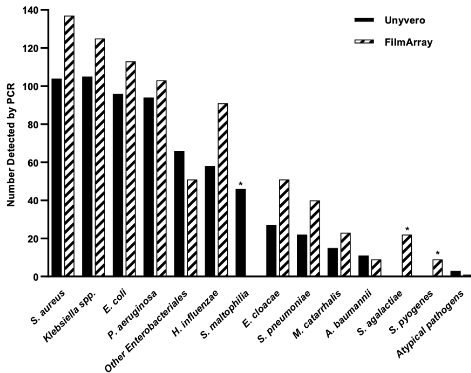
Figure 3b. Numbers and type of bacteria detected by PCR from respiratory samples included in the study. Unyvero, solid bars, n = 606; FilmArray, hatched bars, n = 620. Species sought by one test only are marked with an asterisk.
