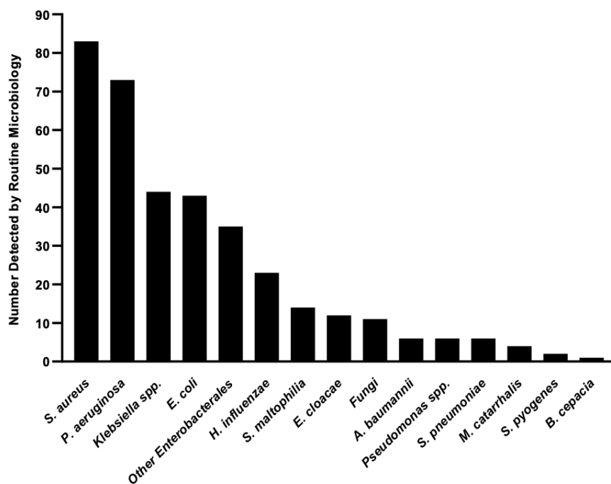
Figure 3a. Numbers and types of bacteria detected by RM culture from respiratory samples included in the study.
