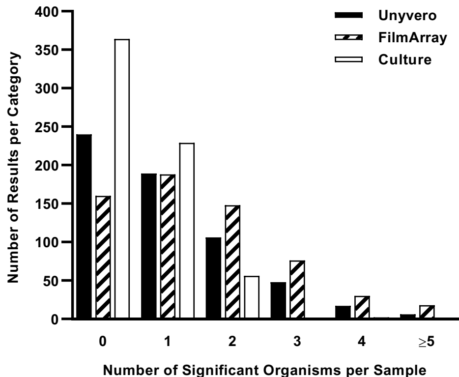
Figure 2. Number of significant organisms detected per respiratory sample by RM or PCR.
