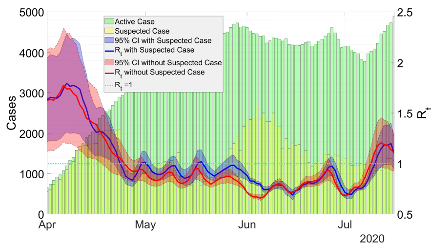
Figure 4: Estimation of \mathcal{R}_t with and without suspected cases.
