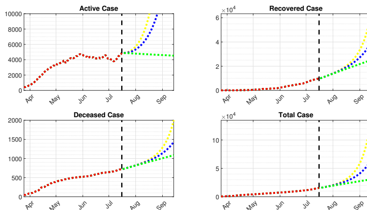
Figure 7: Forecast with different scenarios.
