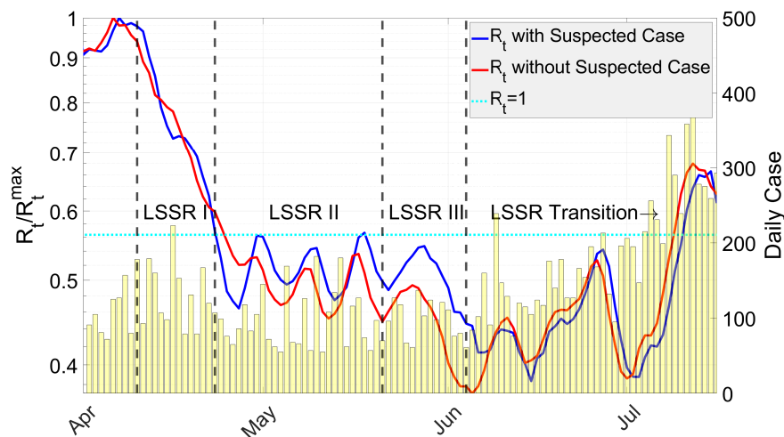
Figure 5: Mean of \mathcal{R}_t/\mathcal{R}_t^{\max} plotted in semi-log scale.
