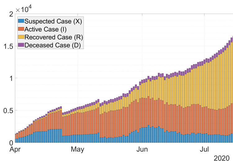
Figure 1: Stacked-bar of COVID-19 cases in Jakarta, Indonesia.
