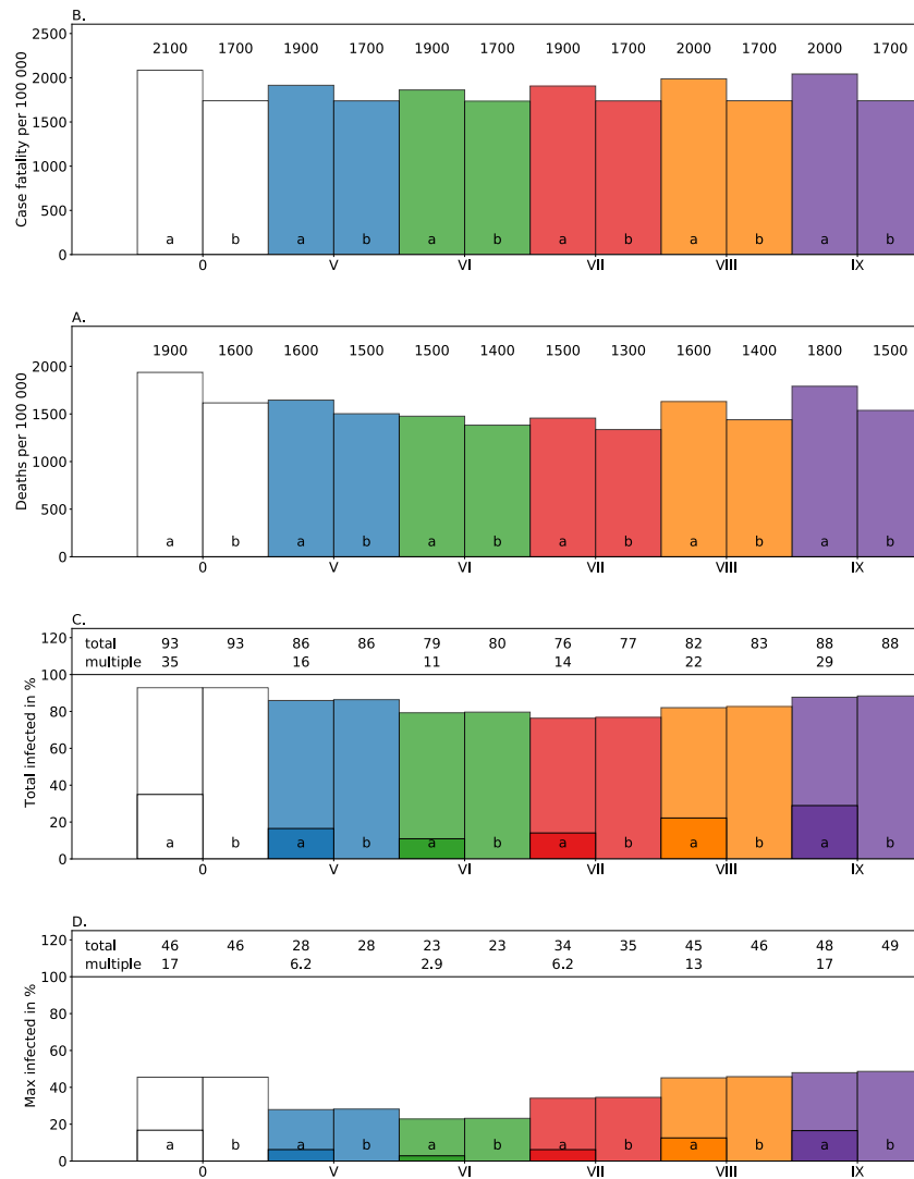
S2 Fig. Implication of a second lockdown. For each scenario (0, V – IX), values are given for the assumption that multi infections cause higher morbidity and mortality and are more likely to be isolated than single infections as described in the text (a) and for the assumption that morbidity, mortality and isolation are the same as for single infection (b). Shown are the total number of deaths (A); (B) case fatality (i.e., deaths per infected individuals); (C) total percentage (of population) being infected or multi infected; and (D) the maximal number of individuals infected or multi infected at the epidemic peak, for scenarios as specified in Table 2 contrasting the case with increased morbidity and mortality of multi infections (a) and no effect of multi infections on mortality and morbidity (b), i.e., the case in which single and multi infections are indistinguishable. The horizontal lines in scenario (a) in (C) and (D) indicate the number of multi infections characterized by increased morbidity and mortality given by (33) in S1 Appendix. Parameters are given in S1 Table – S4 Table.
