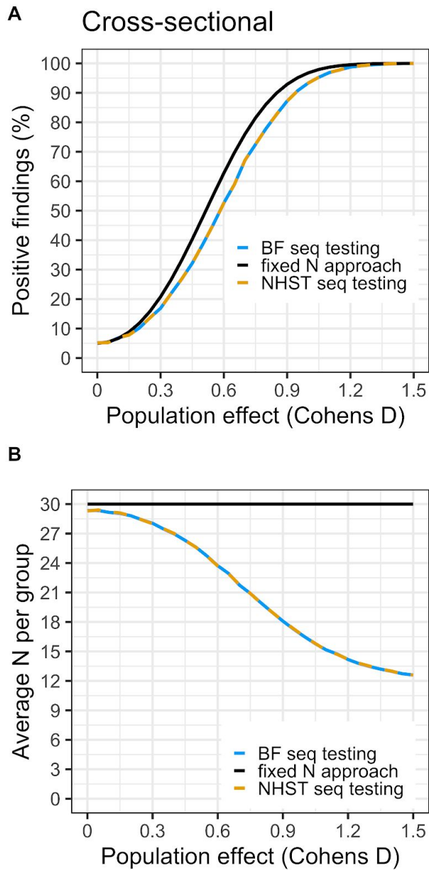
Figure S2. The sequential BF testing, using a zero-centered Cauchy to describe the alternative hypothesis, will produce the same results as a 5% family-wise error rate corrected sequential NHST procedure when specifying the BF threshold to correspond to a 5% false positive rate ( BF = 4 ).
