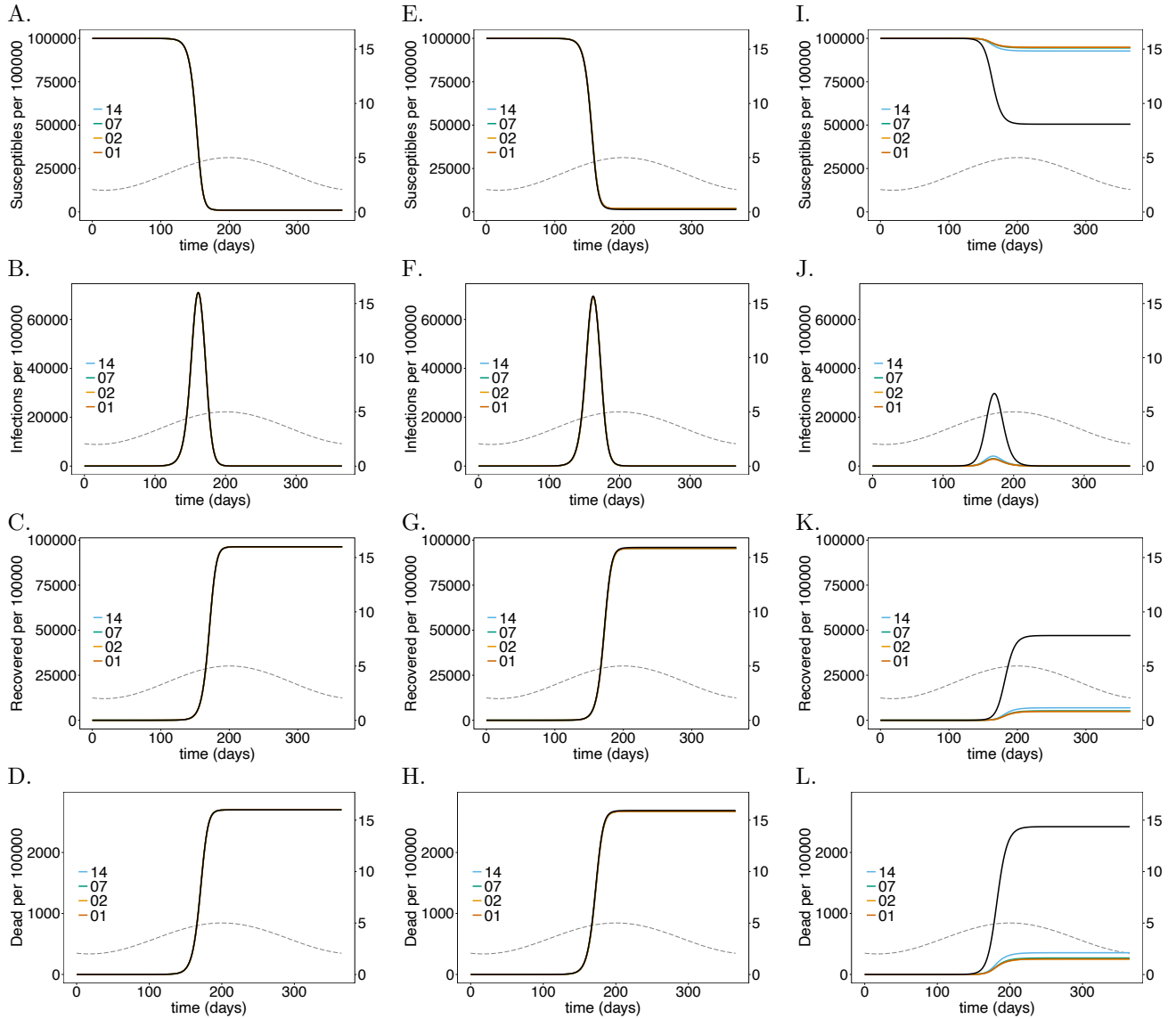
Fig 4. Testing rate assuming seasonal fluctuations: The panels show the number of susceptible ( S ), infected ( I ), recovered ( R ) and dead ( D ) individuals at time t , respectively, for the general sub-population (A-D), the LTCF staff (E-H), and the risk group (I-L) assuming different testing rates (colors). The black line in all panels corresponds to the baseline model without testing. The parameters used are listed in Tables 1, and S1 Table - S6 Table. Seasonal fluctuations in R_0 are shown by the dashed line (right axis).
