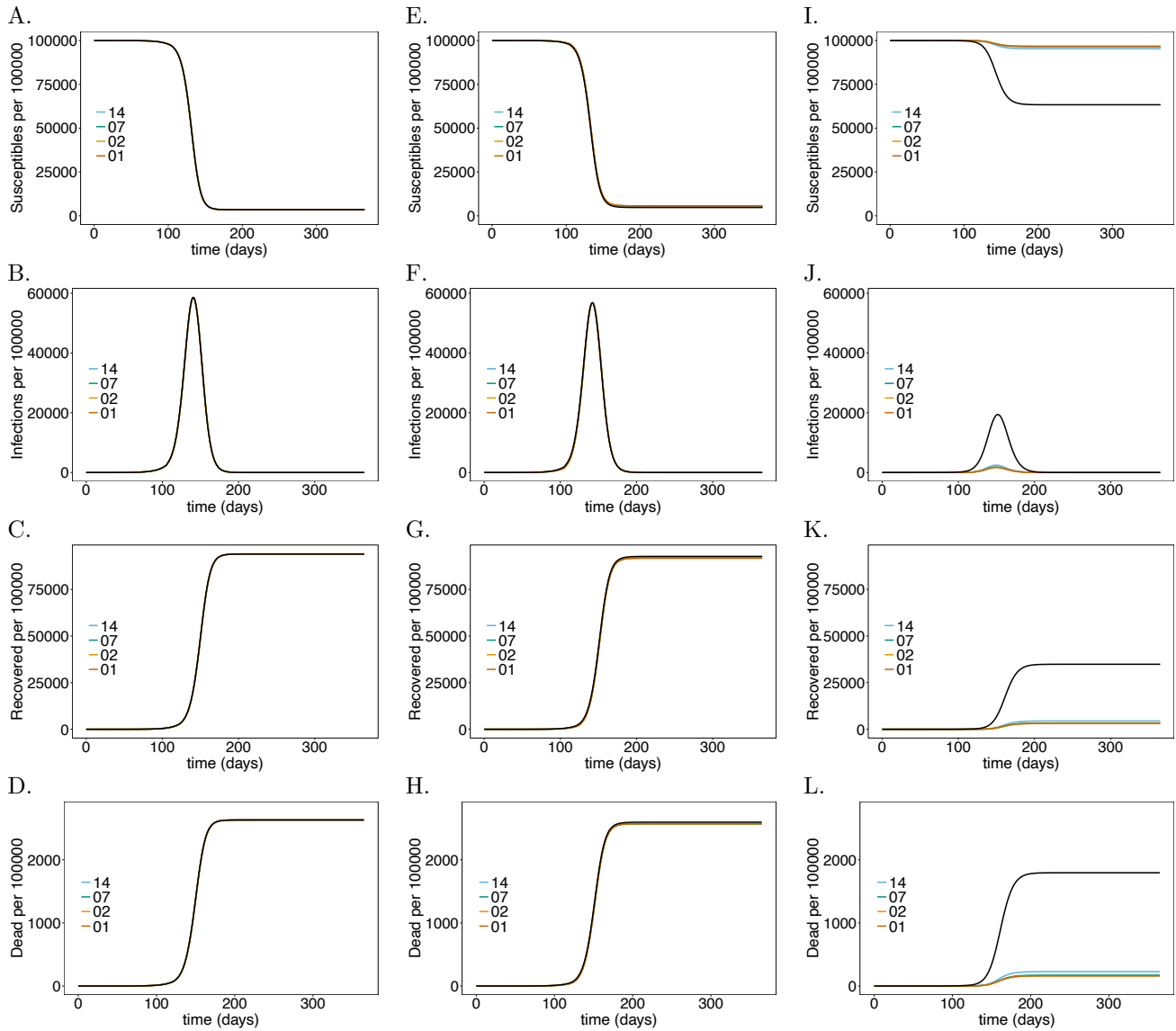
Fig 3. Testing rate without seasonal fluctuations: The panels show the number of susceptible ( S ), infected ( I ), recovered ( R ) and dead ( D ) individuals at time t , respectively, for the general sub-population (A-D), the LTCF staff (E-H), and the risk group (I-L) assuming different testing rates (colors). The black line in all panels corresponds to the baseline model without testing. The parameters used are listed in Tables 1, and S1 Table - S6 Table, no seasonal fluctuations in R_0 are assumed.
