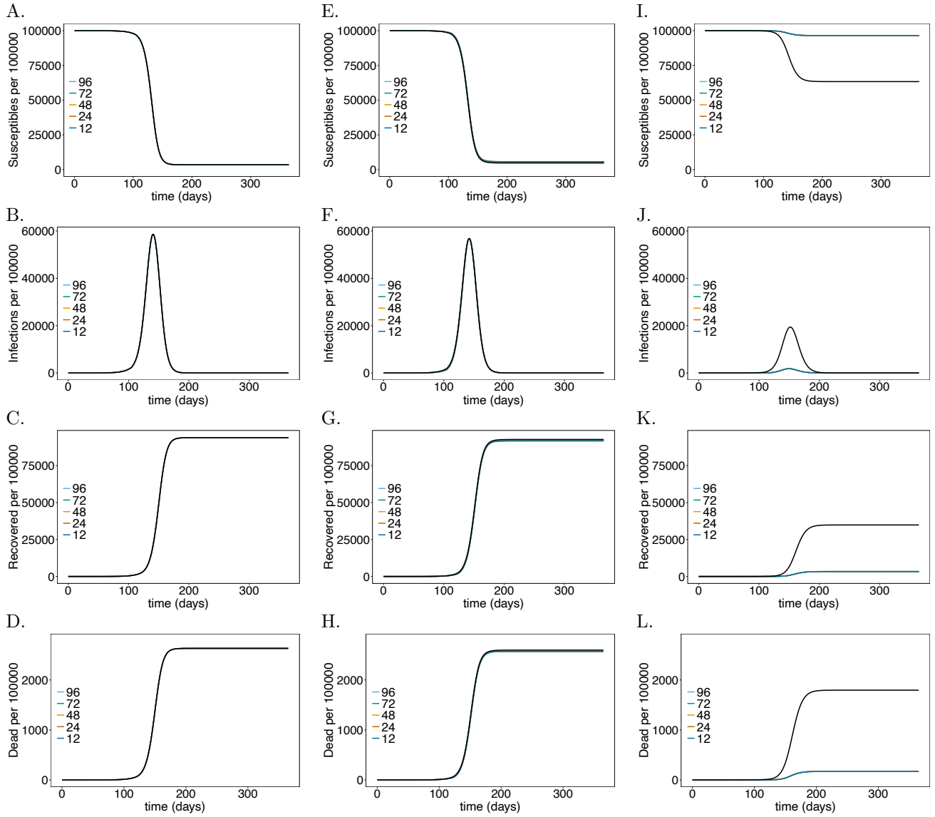
Fig 5. Test-processing time without seasonal fluctuations: The panels show the number of infected ( I ), susceptible ( S ), recovered ( R ) and dead ( D ) individuals at time t , respectively, for the general sub-population (A-D), the LTCF staff (E-H), and the risk group (I-L) assuming different processing times in hours (colors). The black line in all panels corresponds to the baseline model without testing. The parameters used are listed in Tables 1, and S1 Table - S6 Table, no seasonal fluctuations in R_0 are assumed.
