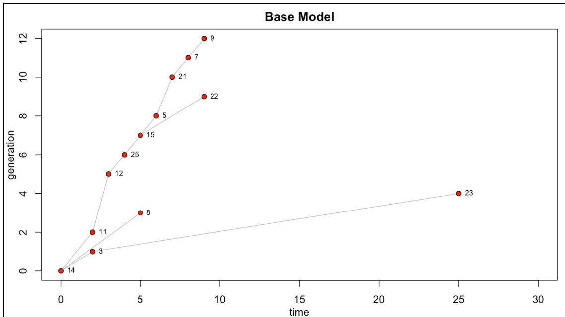
Supplemental Figure 1. The Forward Reachable Path for Node 14 in the Base Model (With Concurrency) of 25 Nodes Simulated for 25 Time Steps.
