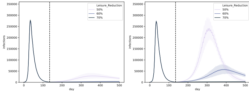
Figure 7: Trends for different leisure contact reductions, when performing weekly universal testing, and importing 10 cases per day. We assume that universal testing starts on the first of July and that FNR_{PCR} = 0.1 . We consider both isolation strategies: pool isolation (left panel) and individual isolation (right panel). The curves show a line that depicts the average over the trajectories of the result aggregations and a shaded area that depicts the standard deviation.
