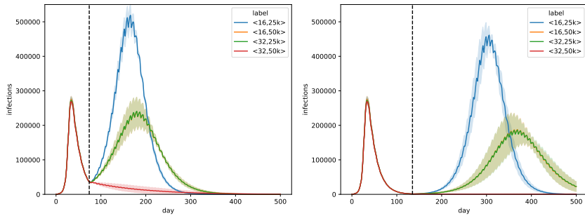
Figure 3: Trends for individual isolation. Trends for all combinations of parameters \langle k, T_d \rangle , for \text{FNR}_{\text{PCR}} = 0.1 . Universal testing starts at the first of May (left panel) and the first of July (right panel). We follow the individual isolation strategy, where we identify the infected individuals in positive pool. The curves show a line that depicts the average over the trajectories of the result aggregations and a shaded area that depicts the standard deviation. Note that in this figure, the orange and green curve overlap.
