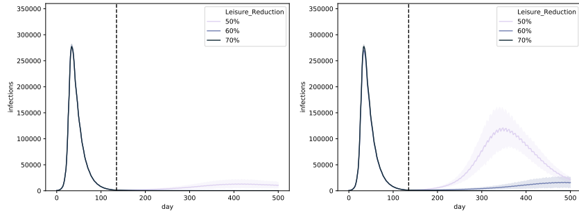
Figure 15: Simulated epidemic curves for different leisure contact reductions, when performing weekly universal testing. We assume that universal testing starts on the first of July and that \text{FNR}_{\text{PCR}} = 0.05 . We consider both isolation strategies: pool isolation (left panel) and individual isolation (right panel). The curves show a line that depicts the average over the trajectories of the result aggregations and a shaded area that depicts the standard deviation.
