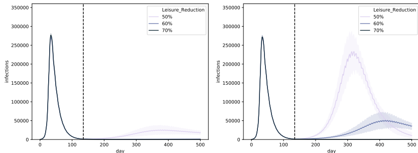
Figure 6: Trends for different leisure contact reductions, when performing weekly universal testing. We assume that universal testing starts on the first of July and that \text{FNR}_{\text{PCR}} = 0.1 . We consider both isolation strategies: pool isolation (left panel) and individual isolation (right panel). The curves show a line that depicts the average over the trajectories of the result aggregations and a shaded area that depicts the standard deviation.
