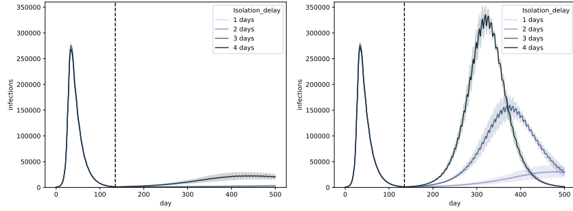
Figure 22: Sensitivity analysis for weekly universal testing ( k = 32 , T_d = 50k ) with a contact reduction of 70%, considering d_t = \{1, 2, 3, 4\} . We assume that universal testing starts on the first of July and that \text{FNR}_{\text{PCR}} = 0.1 . We consider both isolation strategies: pool isolation (left panel) and individual isolation (right panel). The curves show a line that depicts the average over the trajectories of the result aggregations and a shaded area that depicts the standard deviation.
