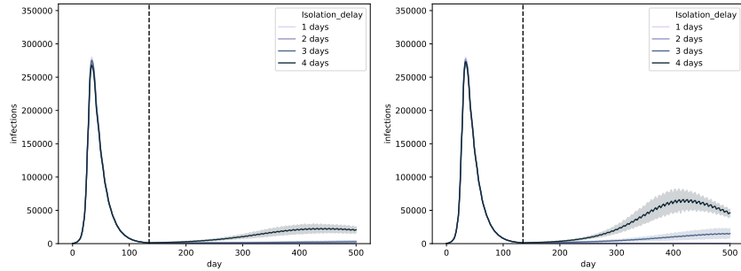
Figure 23: Sensitivity analysis for weekly universal testing ( k = 32 , T_d = 50k ) with a contact reduction of 70%, considering d_t = \{1, 2, 3, 4\} . We assume that universal testing starts on the first of July and that \text{FNR}_{\text{PCR}} = 0.1 . We consider both isolation strategies: pool isolation (left panel) and household isolation (right panel). The curves show a line that depicts the average over the trajectories of the result aggregations and a shaded area that depicts the standard deviation.
