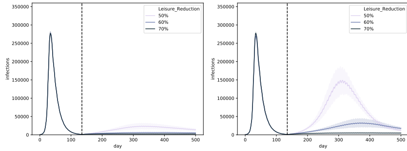
Figure 17: Simulated epidemic curves for different leisure contact reductions, when performing weekly universal testing, and importing 50 cases per day. We assume that universal testing starts on the first of July and that FNR_{PCR} = 0.05 . We consider both isolation strategies: pool isolation (left panel) and individual isolation (right panel). The curves show a line that depicts the average over the trajectories of the result aggregations and a shaded area that depicts the standard deviation.
