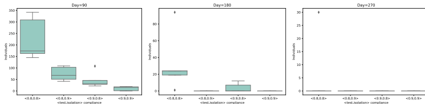
Figure 4: Distribution for pool isolation. Distribution of the number of infections for the experiment when the lock-down ends on the first of July, in different scenarios of compliance for testing and isolation. We show the number of infections at three different time points. i.e., 90 days (left panel), 180 days (middle panel) and 270 days (right panel) after the start of the universal testing procedure. These results consider a weekly universal testing procedure (i.e., k = 32 and T_d = 50000 ) and a FNR_{PCR} = 0.1 , where the isolation strategy is pool isolation. Each box represents a combination of test and isolation compliance.
