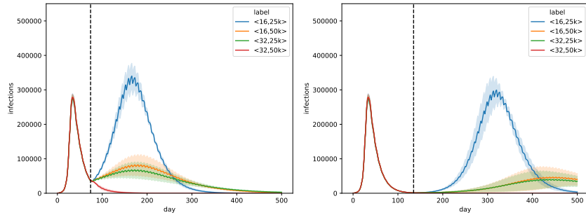
Figure 11: Trends for pool isolation. Simulated epidemic curves for all combinations of parameters \langle k, T_d \rangle , for \text{FNR}_{\text{PCR}} = 0.05 . Universal testing starts at the first of May (left panel) and the first of July (right panel). We follow the isolation strategy where we isolate all individuals that are part of an infected pool. The curves show a line that depicts the average over the trajectories of the result aggregations and a shaded area that depicts the standard deviation.
