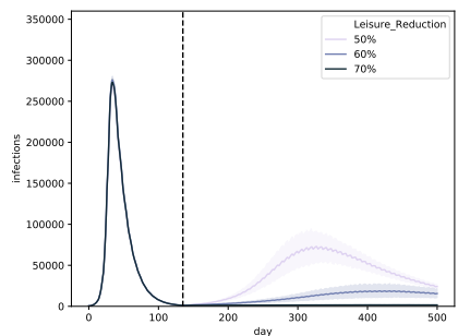
Figure 20: Trends for different leisure contact reductions, when performing weekly universal testing, and importing 10 cases per day. We assume that universal testing starts on the first of July and that FNR_{PCR} = 0.1 . We consider pool isolation and challenge the assumption of household isolation. The curves show a line that depicts the average over the trajectories of the result aggregations and a shaded area that depicts the standard deviation.
