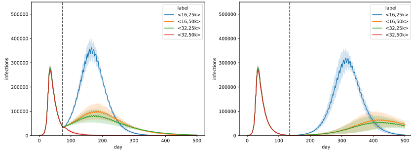
Figure 2: Trends for pool isolation. Trends for all combinations of parameters \langle k, T_d \rangle , for \text{FNR}_{\text{PCR}} = 0.1 . Universal testing starts at the first of May (left panel) and the first of July (right panel). We follow the pool isolation strategy, where we isolate all individuals that are part of an infected pool. The curves show a line that depicts the average over the trajectories of the result aggregations and a shaded area that depicts the standard deviation.
