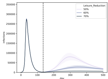
Figure 21: Trends for different leisure contact reductions, when performing weekly universal testing, and importing 50 cases per day. We assume that universal testing starts on the first of July and that FNR_{PCR} = 0.1 . We consider pool isolation and challenge the assumption of household isolation. The curves show a line that depicts the average over the trajectories of the result aggregations and a shaded area that depicts the standard deviation.
