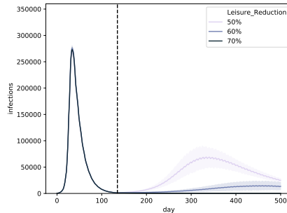
Figure 19: Trends for different leisure contact reductions, when performing weekly universal testing. We assume that universal testing starts on the first of July and that \text{FNR}_{\text{PCR}} = 0.1 . We consider pool isolation and challenge the assumption of household isolation. The curves show a line that depicts the average over the trajectories of the result aggregations and a shaded area that depicts the standard deviation.
