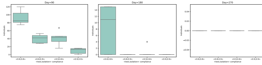
Figure 13: Distribution for pool isolation. Distribution of the number of infections for the experiment when the lock-down end on the first of July, in different scenarios of compliance for testing and isolation. We show the number of infections at three different time points. i.e., 90 days (left panel), 180 days (middle panel) and 270 days (right panel) after the start of the universal testing procedure. These results consider a weekly universal testing procedure (i.e., k = 32 and T_d = 50000 ) and a FNR_{PCR} = 0.05 , where the isolation strategy is pool isolation. Each box represents a combination of test and isolation compliance.
