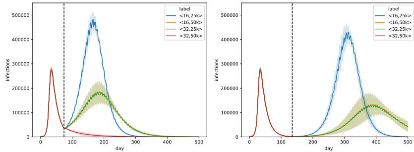
Figure 12: Trends for individual isolation. Simulated epidemic curves for all combinations of parameters \langle k, T_d \rangle , for \text{FNR}_{\text{PCR}} = 0.05 . Universal testing starts at the first of May (left panel) and the first of July (right panel). We follow the isolation strategy where we identify the infected individuals in the positive pool. The curves show a line that depicts the average over the trajectories of the result aggregations and a shaded area that depicts the standard deviation.
