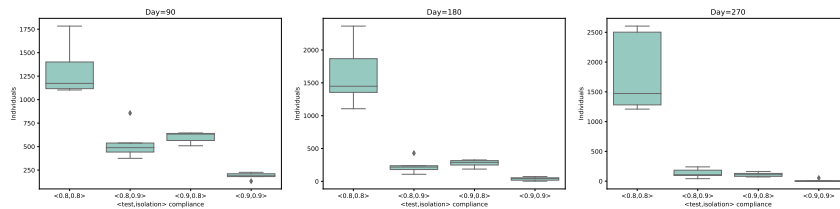
Figure 5: Distribution for pool isolation. Distribution of the number of infections for the experiment when the lock-down ends on the first of July, in different scenarios of compliance for testing and isolation. We show the number of infections at three different time points. i.e., 90 days (left panel), 180 days (middle panel) and 270 days (right panel) after the start of the universal testing procedure. These results consider a weekly universal testing procedure (i.e., k = 32 and T_d = 50000 ) and a \text{FNR}_{\text{PCR}} = 0.1 , where the isolation strategy is individual isolation. Each box represents a combination of test and isolation compliance.
