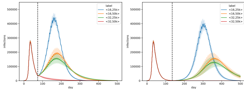
Figure 18: Trends for all combinations of parameters \langle k, T_d \rangle , for \text{FNR}_{\text{PCR}} = 0.1 . Universal testing starts at the first of May (left panel) and the first of July (right panel). We follow the pool isolation strategy, where we isolate all individuals that are part of an infected pool. The curves show a line that depicts the average over the trajectories of the result aggregations and a shaded area that depicts the standard deviation.
