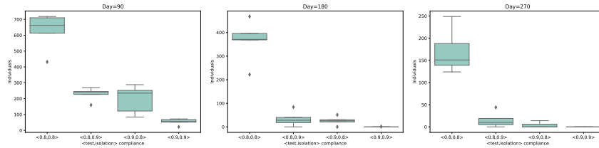
Figure 14: Distribution for individual isolation. Distribution of the number of infections for the experiment when the lock-down end on the first of July, in different scenarios of compliance for testing and isolation. We show the number of infections at three different time points. i.e., 90 days (left panel), 180 days (middle panel) and 270 days (right panel) after the start of the universal testing procedure. These results consider a weekly universal testing procedure (i.e., k = 32 and T_d = 50000 ) and a FNR_{PCR} = 0.05 , where the isolation strategy is individual isolation. Each box represents a combination of test and isolation compliance.
