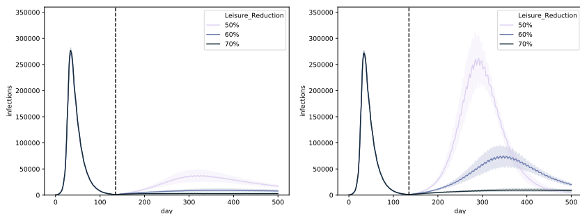
Figure 8: Trends for different leisure contact reductions, when performing weekly universal testing, and importing 50 cases per day. We assume that universal testing starts on the first of July and that FNR_{PCR} = 0.1 . We consider both isolation strategies: pool isolation (left panel) and individual isolation (right panel). The curves show a line that depicts the average over the trajectories of the result aggregations and a shaded area that depicts the standard deviation.
