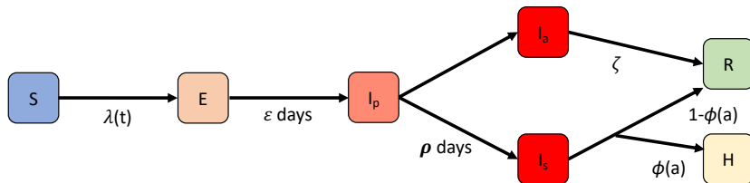
Figure 1: We consider that an individual goes through different phases of infection/disease, which is represented by a SEIR-like state machine. A susceptible individual ( S ) can become infected, given a time-dependent infection probability \lambda(t) . This probability depends on the transmission potential of the virus and the social contact behaviour, which due to contact reduction policies is time-dependent. When infected, the individual becomes exposed ( E ). Once exposed ( E ), an individual goes through an incubation time of \varepsilon days, after which the individual becomes infectious prior to symptom development ( I_p ). A pre-symptomatic infected individual ( I_p ) will either become asymptomatic ( I_a ), symptomatic with symptoms ( I_s ), after a period of \rho days. When asymptomatic ( I_a ) the individual will remain infectious for \zeta days after which he/she recovers ( R ). When severely symptomatic, the individual will be hospitalized with an age-dependent probability \phi(a) or recover without the need for hospitalisation.
