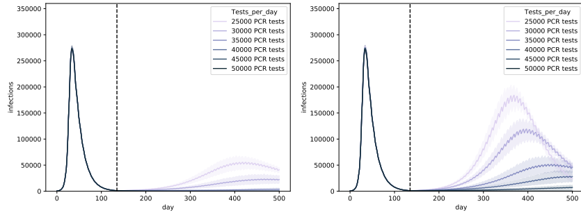
Figure 24: Weekly versus bi-weekly universal testing (i.e., k = 32, T_d \in \{25k, 30k, 35k, 40k, 45k, 50k\} ) with a contact reduction of 70%, considering d_t = \{1, 2, 3, 4\} . We assume that universal testing starts on the first of July and that \text{FNR}_{\text{PCR}} = 0.1 . We consider both isolation strategies: pool isolation (left panel) and individual isolation (right panel). The curves show a line that depicts the average over the trajectories of the result aggregations and a shaded area that depicts the standard deviation.
