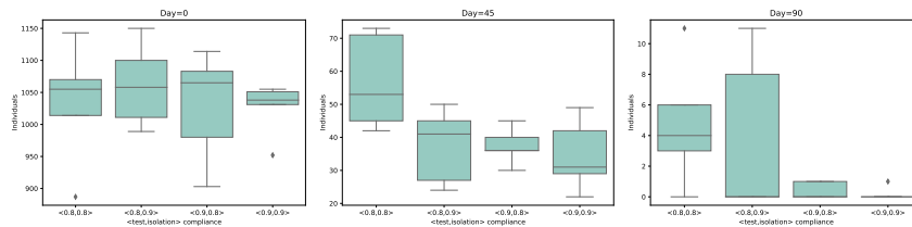
Figure 9: Distribution of the number of infections for the experiment when the lock-down restrictions are continued. We show different scenarios of compliance for testing and isolation. We show the number of infections at three different time points. i.e., 0 days (left panel), 45 days (middle panel) and 90 days (right panel) after the start of the universal testing procedure. These results consider a weekly universal testing procedure (i.e., k = 32 and T_d = 50000 ) and a \text{FNR}_{\text{PCR}} = 0.1 , where the isolation strategy is individual isolation. Each box represents a combination of test and isolation compliance. Note that 135 days after the start of the universal testing procedure (not shown in this figure), the number of cases dropped to zero, for all the compliance scenarios.
