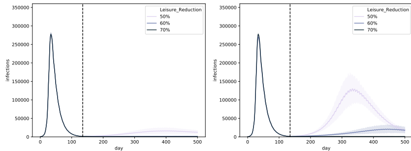
Figure 16: Simulated epidemic curves for different leisure contact reductions, when performing weekly universal testing, and importing 10 cases per day. We assume that universal testing starts on the first of July and that \text{FNR}_{\text{PCR}} = 0.05 . We consider both isolation strategies: pool isolation (left panel) and individual isolation (right panel). The curves show a line that depicts the average over the trajectories of the result aggregations and a shaded area that depicts the standard deviation.
