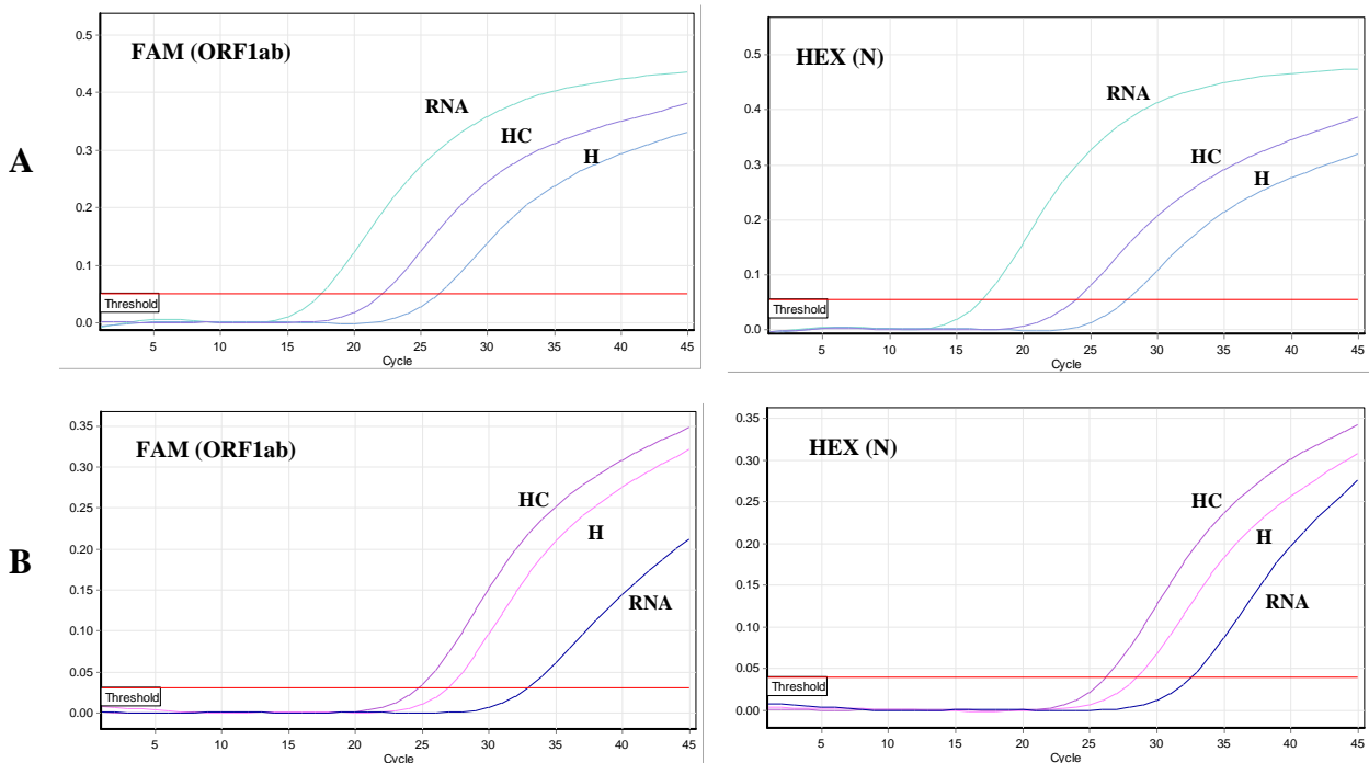
Figure 1. qRT-PCR amplification plots for the SARS-CoV-2 ORF1ab (FAM) and N (HEX) genes for a nasopharyngeal swab sample subjected to the standard RNA extraction, heat inactivation (H), and heat inactivation and pelleting (HC). Amplification plots show normalized value ( \Delta Rn, linear scale) as a function of the qPCR cycle. The horizontal red line denotes the cycle threshold.
