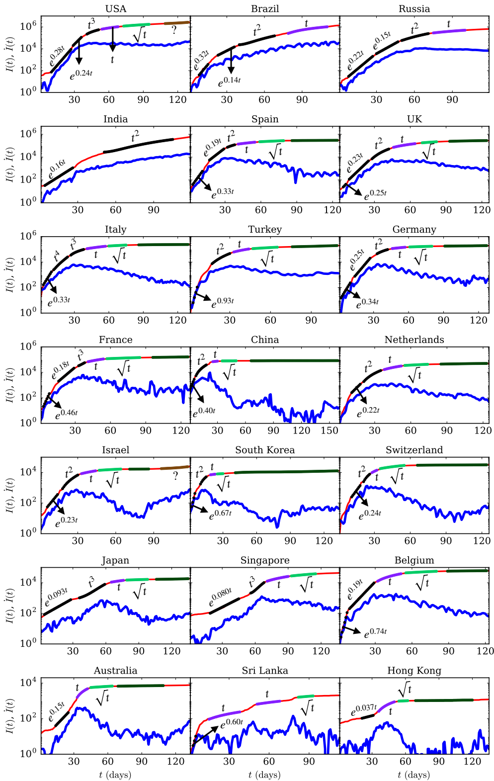
Figure 1: (color online) For the COVID-19 epidemic, the semi-logy plots of total infected individuals ( I(t) ) vs. time ( t ) (red curves) for 21 countries. We also plot \dot{I}(t) vs. t (blue curves). The dotted curves represent the best-fit curves, which are exponential or polynomial functions (see Table 1). The dark-green curves represent the flattened regions of the epidemic.
