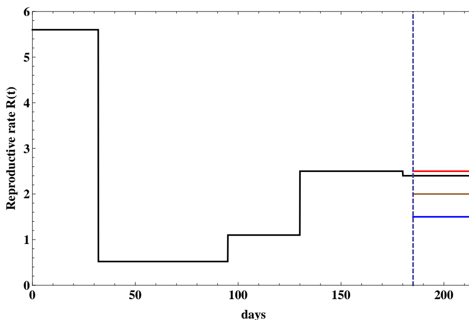
Figure 2: Change in the reproduction transmission factor R(t) as a function of time t (in days) in Lebanon. It starts at R_0 = 5.6 then falls down at t = 32 days to R_1 = 0.52 after strong mitigation measures. It rises to R_2 = 1.1 at t = 95 days then to R_3 = 2.5 at t = 130 days, before a slight decrease into R_4 = 2.4 between t = 180 and t = 186 . The four future possible scenarios inspected here have values of R_t = R_5 = 1.5, 2, 2.4 or 2.5 after t = 186 represented in blue, brown, black and red respectively.
