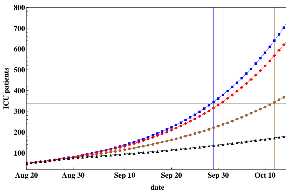
Figure 3: Expected number of ICU patients until the middle of October, according to the different scenarios. The number of ICU patients would exceed the number of all available ICU beds (336 beds represented by the horizontal black line), on September 29, October 1, October 12 for R_5 = 2.5, 2, 4 or 2 respectively. In case of severe measures with R_5 = 1.5 , the number of patients in need of ICU would be at nearly half the number of available beds by mid October.
