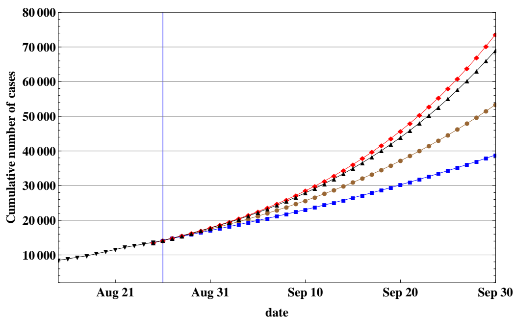
Figure 1: Cumulative number of infections according to the STEIR model in Lebanon, with appropriate parameterization of R_t . The vertical blue line corresponds to day 186, which occurs on August 26, 2020. The black line before represents actually registered cases until that date, while the following four blue, brown, black and red lines correspond to future predictions based on four different scenarios with R_t = 1.5, 2, 2.4 or 2.5 depending on the extent of relaxation.
