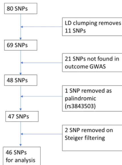
Figure E8. Flow Chart of analysis for effect FEV 1 /FVC SNPs
