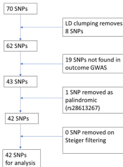
Figure E7. Flow Chart of analysis for FVC SNP's
