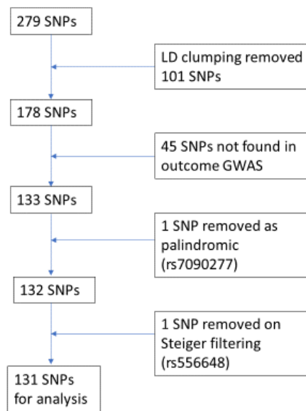
Figure E6. Flow chart of analysis for FEV 1 SNPs
