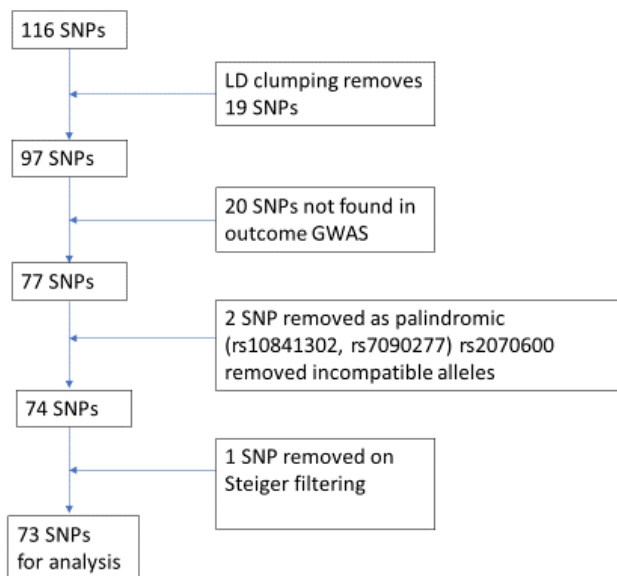
Figure E9. Flow Chart of analysis for COPD liability SNPs (2)
