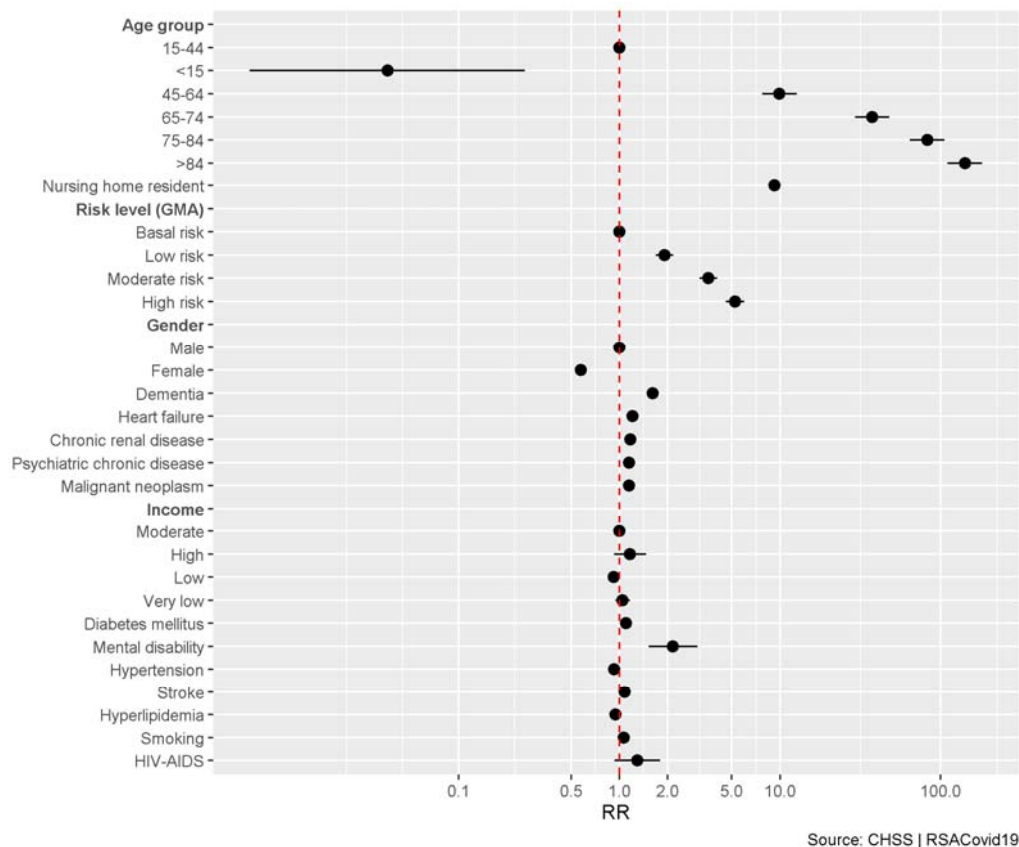
Figure 4. Risk ratios (shown on a log scale) and 95% confidence intervals for each potential risk factor of death by COVID-19 from a Poisson regression model. Data collected in Catalonia, Spain, between 01/03/2020 and 01/06/2020. GMA: adjusted morbidity groups; COVID-19: coronavirus disease 2019; COPD: chronic obstructive pulmonary disease. Gender is considering male as reference.
