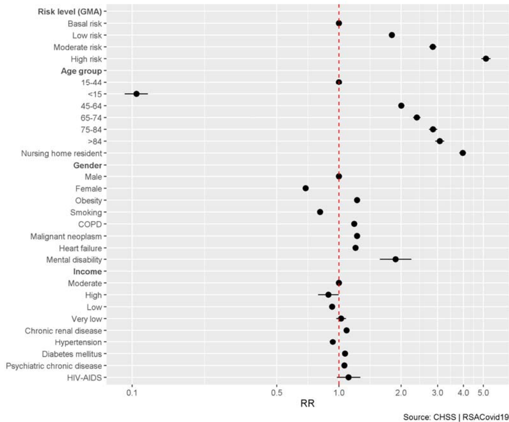
Figure 3. Risk ratios (shown on a log scale) and 95% confidence intervals for each potential risk factor of hospitalisation by COVID-19 from a Poisson regression model. Data collected in Catalonia, Spain, between 01/03/2020 and 01/06/2020. GMA: adjusted morbidity groups; COVID-19: coronavirus disease 2019; COPD: chronic obstructive pulmonary disease. Gender is considering male as reference.
