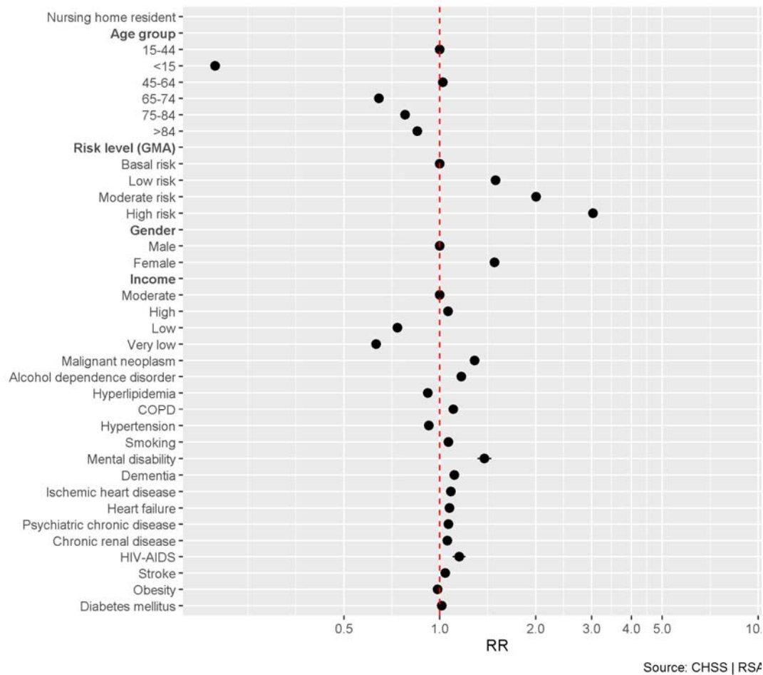
Figure 2. Risk ratios (shown on a log scale) and 95% confidence intervals for each potential risk factor of SARS-CoV-2 diagnosis from a Poisson regression model. Data collected in Catalonia, Spain, between 01/03/2020 and 01/06/2020.
