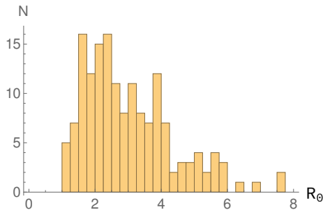
Figure 1.7: Histogram of those values of R_0 which have a standard deviation less than 10% truncated at 8; see the Table B.1, Appendix B for the three missing fits beyond 8.
