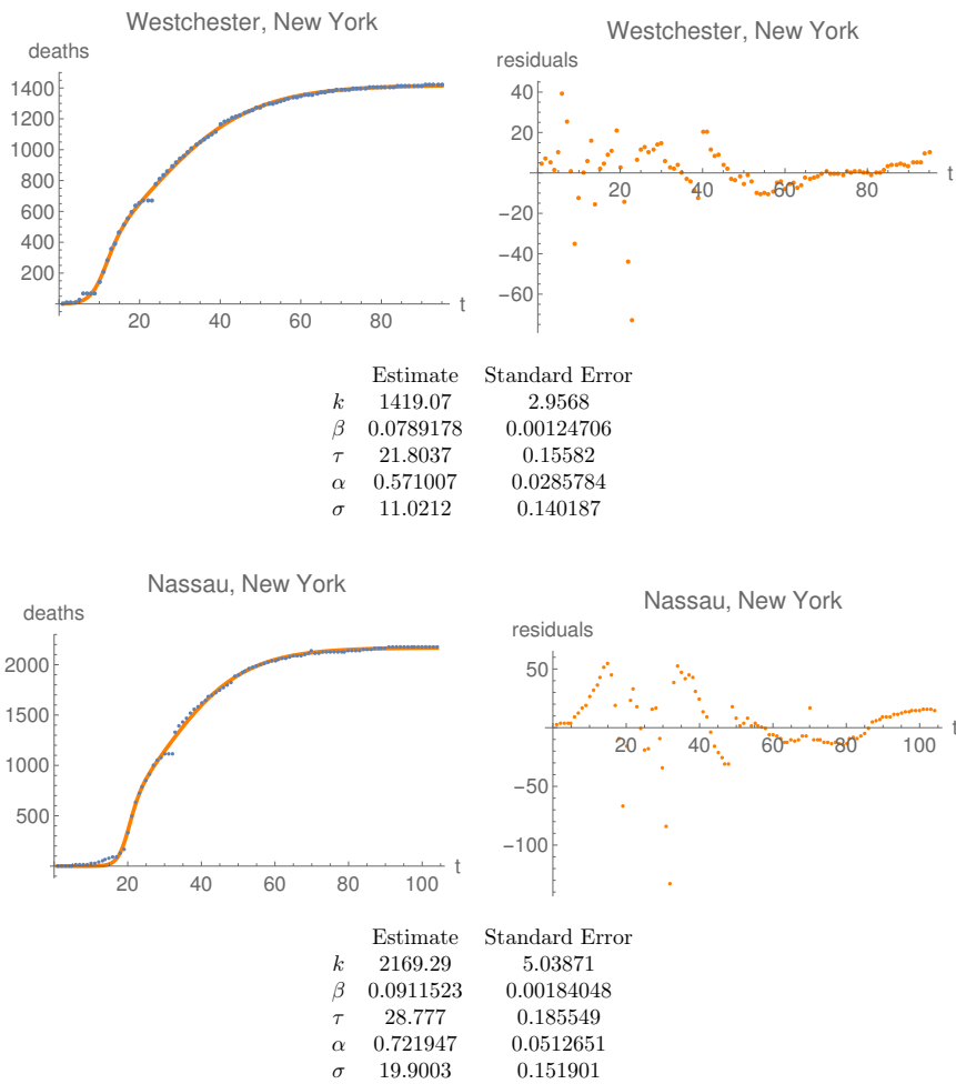
Figure 2.8: Plots of the time series for the best fits before June 30, 2020, and the fit (left), as well as the residuals (right) of the fit for the deaths time-series with largest values of \alpha (Westchester and Nassau Counties, both New York State). One could fine-tune both fits by smoothing out the jumps, which drive the fit down and therefore the residuals up.
