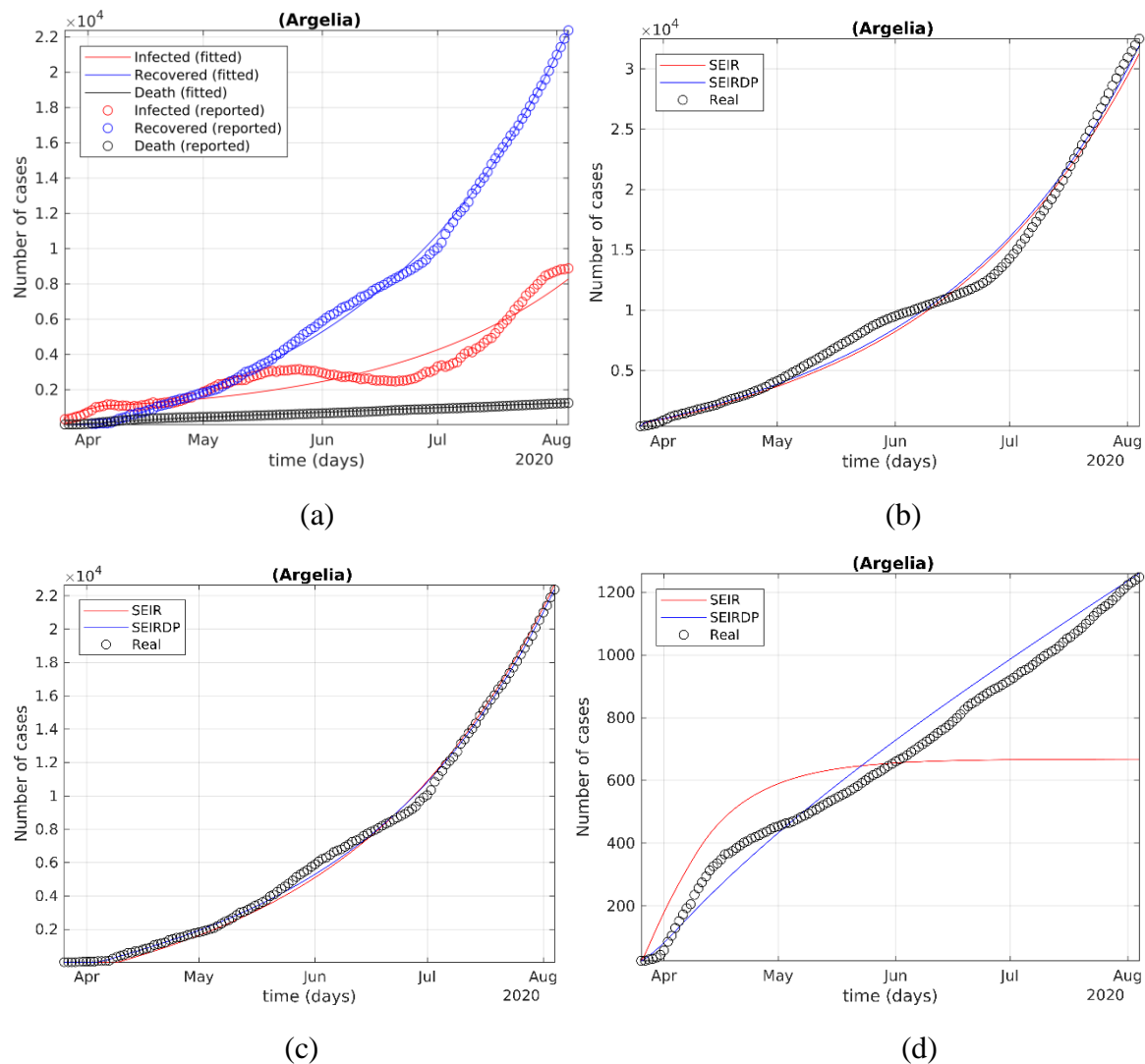
Figure 3: (a) Modeling of the differential SEIRDP model from April 1 to August 3. (c) Modeling of the differential SEIR model from April 1 to August 3 for cumulative positive cases (b), recovered(c) cumulative deaths (d).
