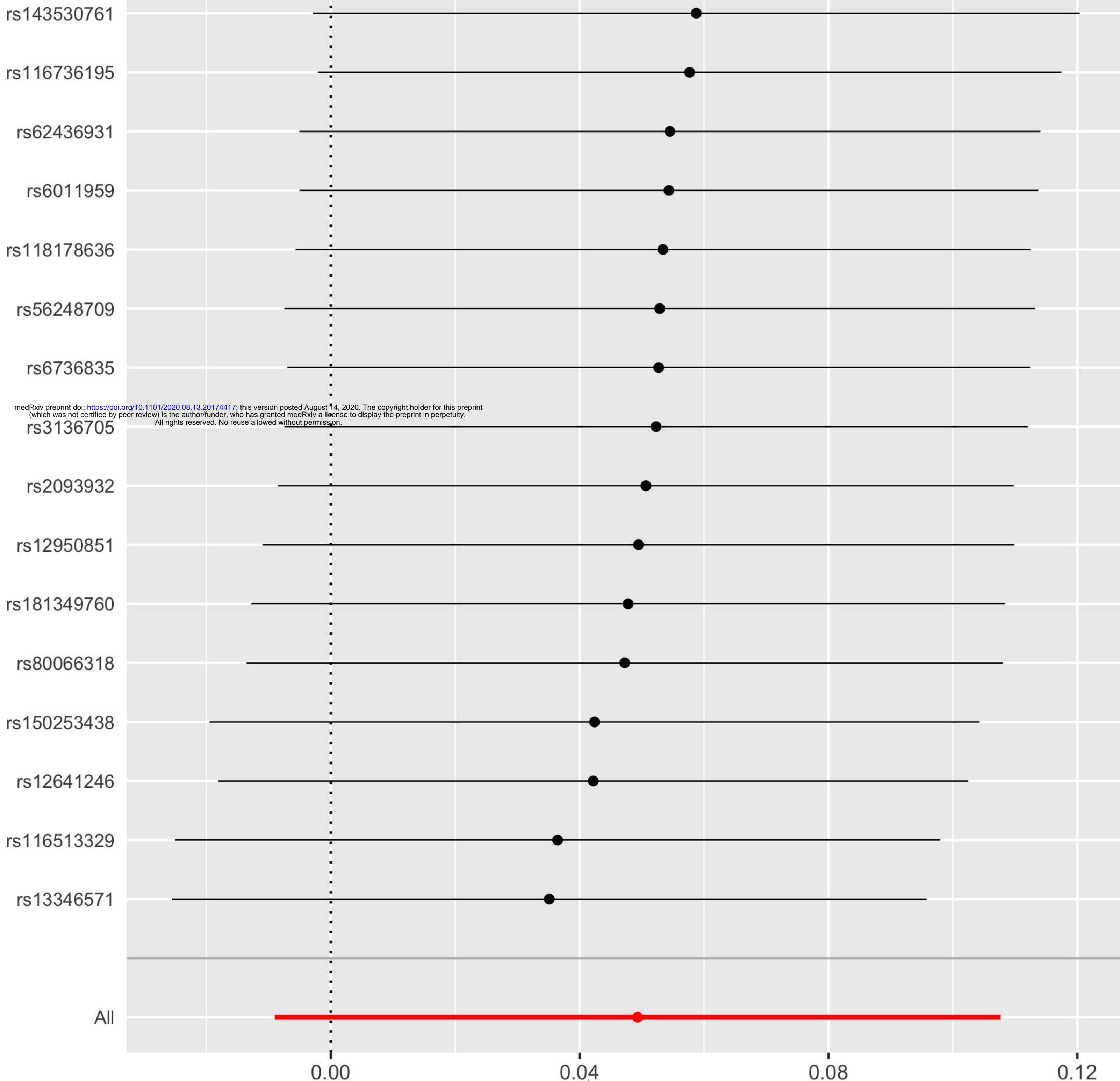
MR leave-one-out sensitivity analysis for COVID-19 on AF
