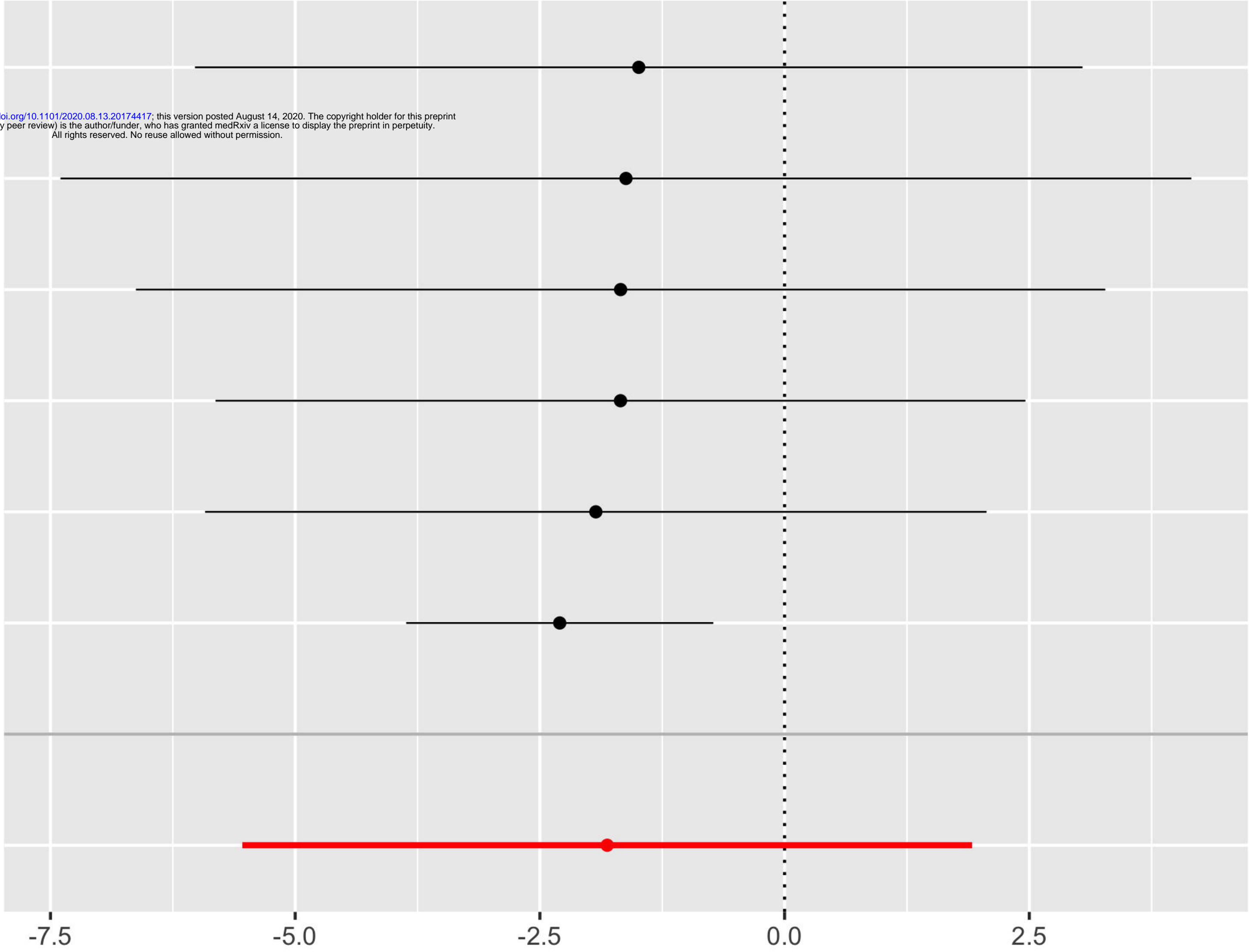
MR leave-one-out sensitivity analysis for AF on COVID-19
