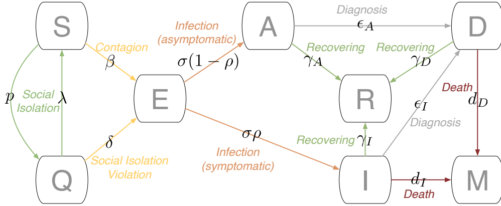
Figure 1: Scheme representing the SINDROME model compartments.
