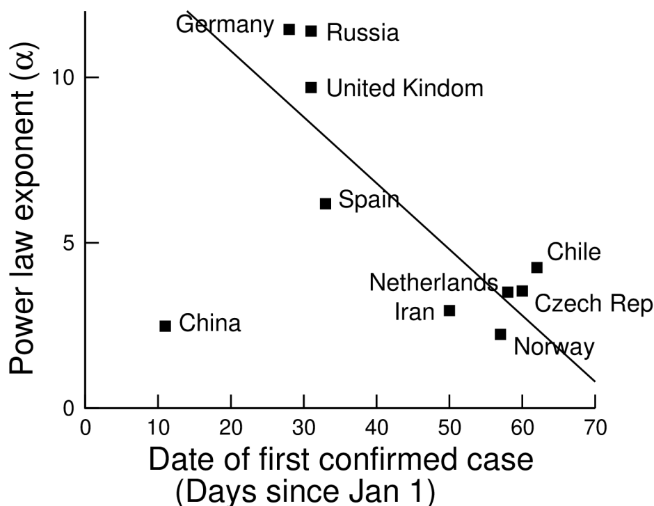
Figure 2. Relationship between the power law exponent and the day of first confirmed case. The points are based on observational data for the COVID-19 outbreak in the indicated countries. The line is the theoretical prediction.
