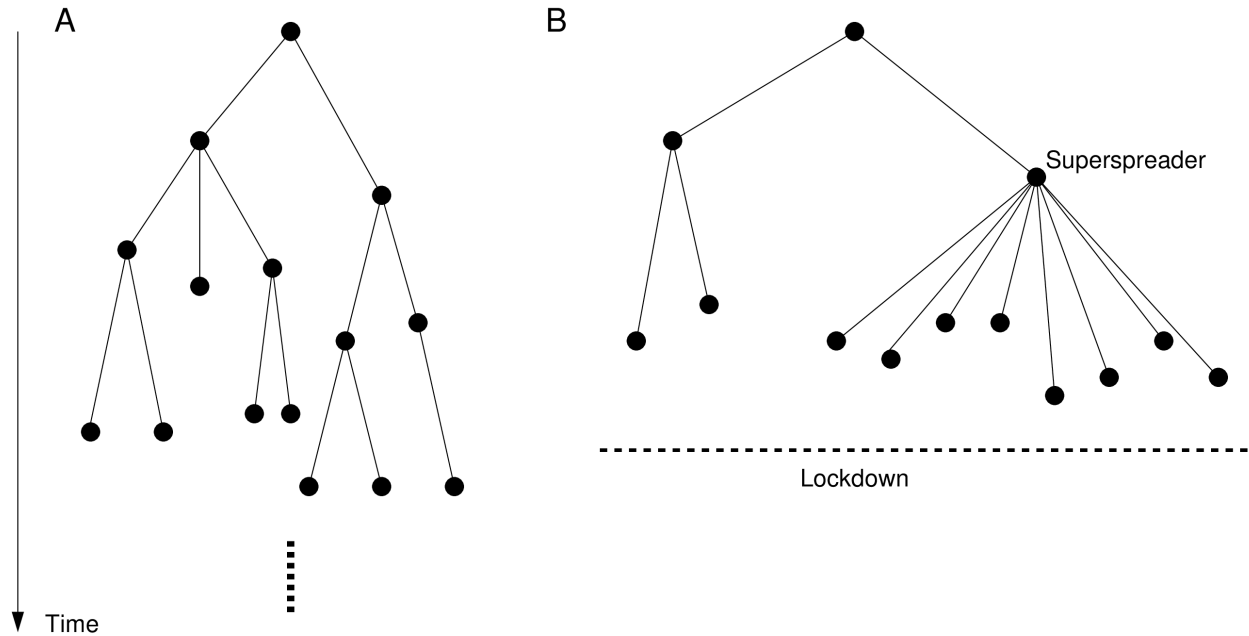
Figure 1. Causal tree of disease transmission of an infectious disease outbreak. A) Typical topology leading to an exponential growth. B) Typical topology leading to a power law growth.
