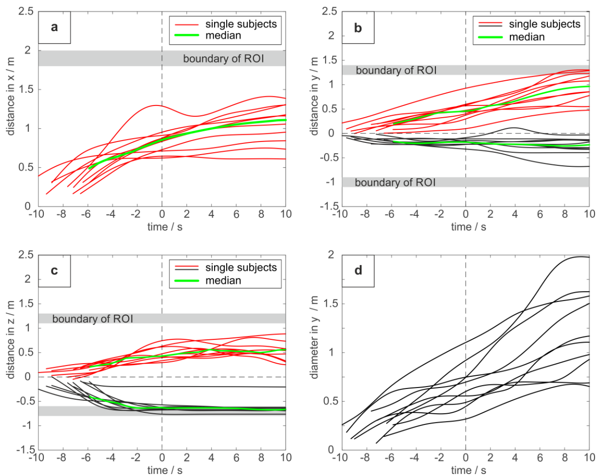
Figure 6: Traces of all subjects for all dimensions (a: x-dimension (front), b: y-dimension (left-right), c: z-dimension (Up-down) and d: diameter of the y-dimension) for the MT+ task. The 0 point in the time-scale refers to the end of the task. The green lines show the median. The corresponding graphs for the other tasks are provided in the supplemental material.
