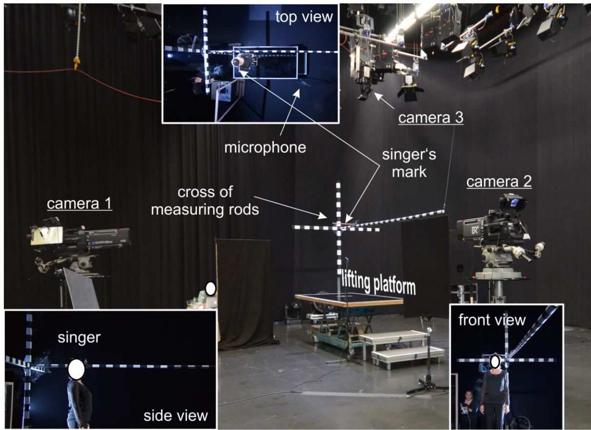
Figure 2: Picture of the test setup including the three cameras, the lifting platform and measuring rod cross (spatial directions are indicated by x, y and z). The perspective views of each camera are shown with a singer in performing position
