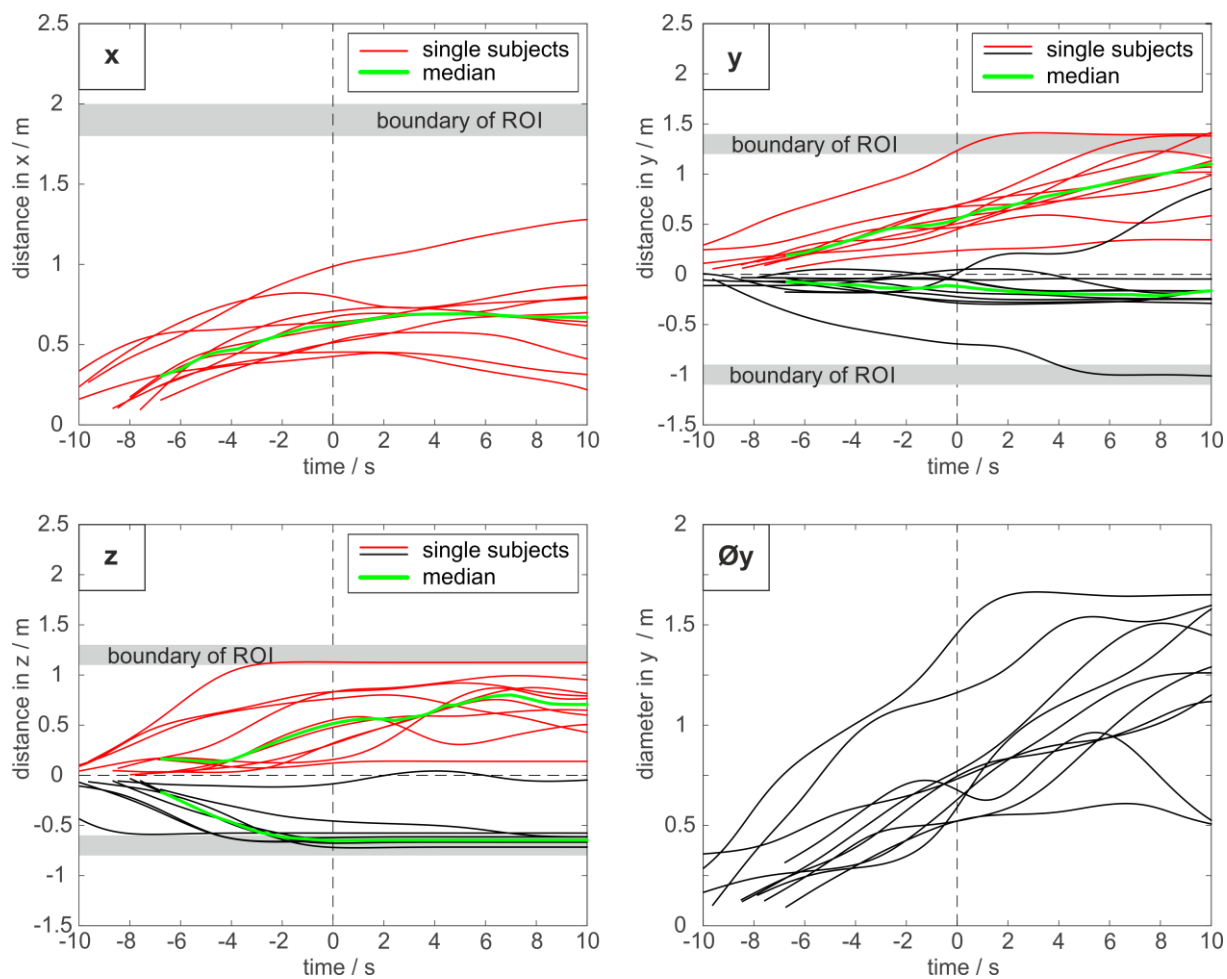
Supplemental Figures 6: Traces of all subjects for all dimensions (a: x-dimension (front), b: y-dimension (left-right), c: z-dimension (Up-down) and d: diameter of the y-dimension) for the M+task. The 0 point in the time-scale refers to the end of the task. The green lines show the median. The corresponding graphs for the other tasks are provided in the supplemental material.
