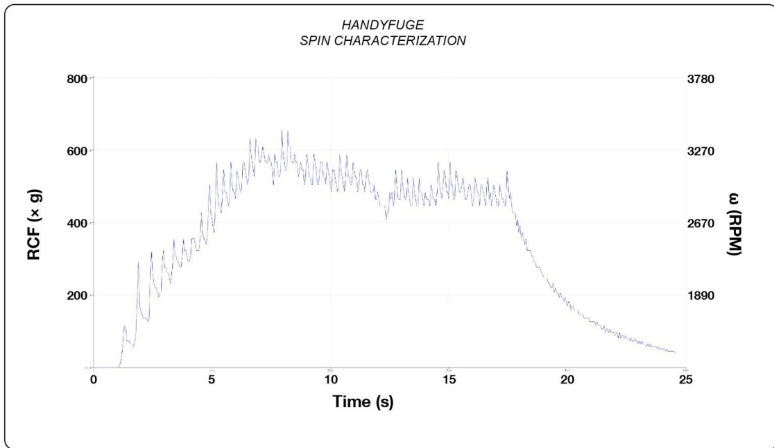
Figure 2. Hall-effect sensor based rotational speed characterization of Handyfuge, demonstrating unidirectional rotation with peak rpm of 3270.
