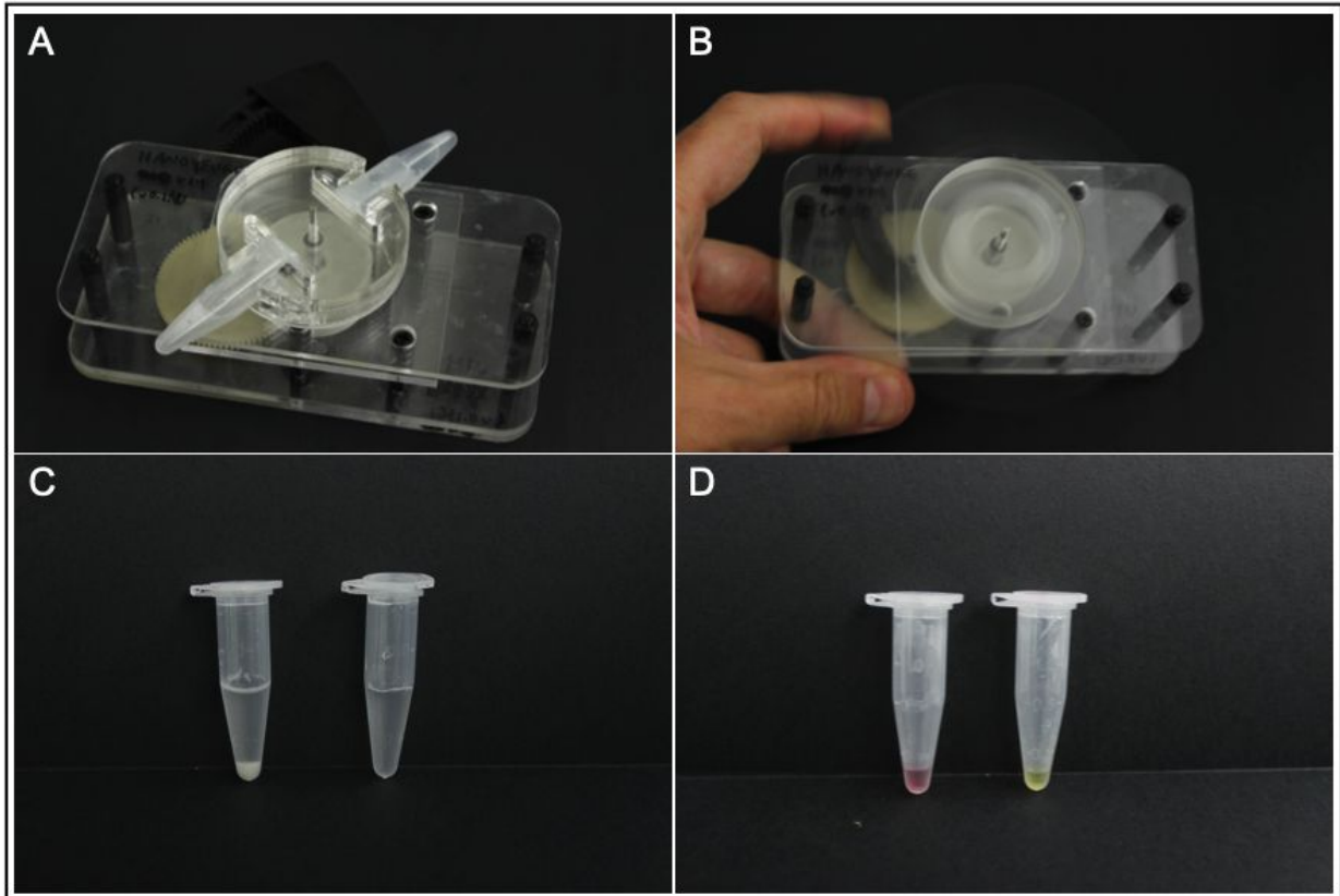
Figure 4. Handyfuge preparation of inhibitor free saliva for LAMP amplification. A) The Handyfuge accepts 2 x 1.5 ml microcentrifuge tubes and a cover for safe operation. B) Hand powered centrifugation can reach sustained speeds of 500RCF. C) Centrifugation at full speed for 1 minute effectively pellets inhibitory flocculant from saliva containing viral RNA. The pelleted flocculant is visible in the tube on the left, the cleared supernatant is on the right. D) After centrifugation, the LAMP protocol can effectively detect synthetic viral RNA down to 10 copies per \mu\text{l} in saliva. The right tube shows the successful amplification of 50,000 COVID control RNA genomes spiked in 500 \mu\text{l} of saliva. The tube on the left was spiked with plasmid DNA as a negative control.
