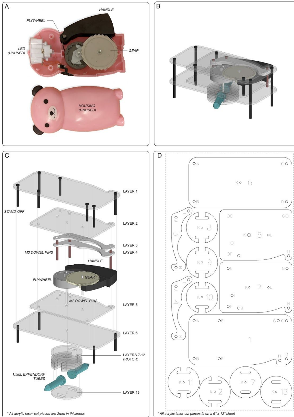
Figure 1. Components of Handyfuge. (A) Dismantled hand-crank flashlight similar to a Dyno-torch flash light providing a one-way ratchet mechanism for converting hand-crank input into uni-directional rotation of the associated gears. (B) Three-dimensional Schematic of a Handyfuge. (C) Assembly and blow-out of of Handyfuge components including borrowed fly-wheel from flash-light and associated acrylic cut pieces. (D) Two-dimensional laser-cut pattern for fabricating a handyfuge.
