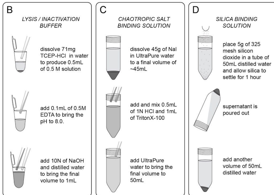
Figure 3. Methods and list of all reagents and steps for Handyfuge-LAMP assay. (A) A picture of all the reagents and tools needed to conduct an electricity-free diagnostics test s. (B)-(D) Preparation of buffers and binding solutions.
