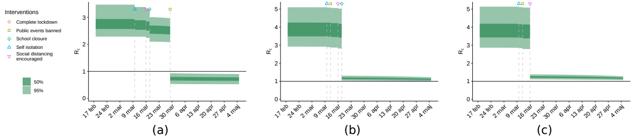
Figure 3. Effect of interventions on virus spread in Sweden, with slightly varying definitions of the interventions. (a) School closure defined to have taken place, public events defined to have been banned on March 29. (b) Same as (a), but with the public events ban moved back to March 12. (c) Same as (b), but with school closure defined not to have taken place. As expected, the visual appearance of the plots is similar, with the last intervention contributing most to the reduction of virus spread. This is problematic, since the last intervention differs between (a), (b), and (c), each relying on equally motivated NPI effectuation dates, de facto introduced by the authors of [2,4] in different versions of the model code [9].
