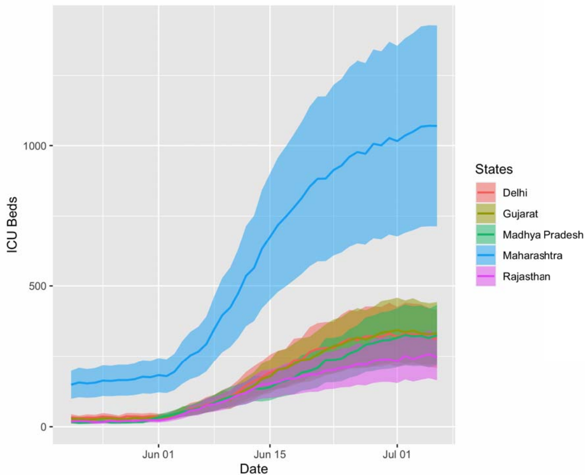
Figure 7: Cumulative ICU beds requirement forecasting from 21 may to 6 july using Agent Based Model
