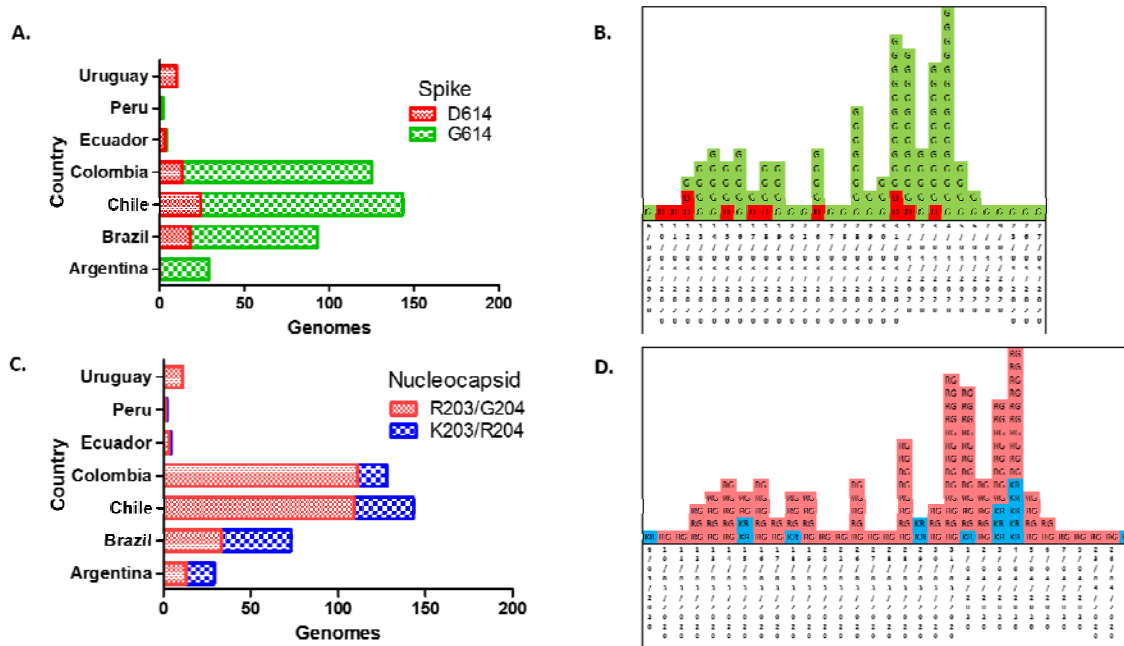
441 Figure 1. Spatiotemporal distribution of the most frequently substitutions in Spike 442 and Nucleocapsid of SARS-CoV-2. A. Distribution of subtypes D614 and G614 of spike 443 protein in SARS-CoV-2 genomes reported as of May 19th, 2020 in Colombia and other 444 South American countries; in red, variant D614 and in green, variant G614. B. Distribution 445 of subtypes D614 and G614 of spike protein in SARS-CoV-2 genomes reported between 446 March and April, 2020 in Colombia, according with the sample collection date, variant 447 D614 and in green, variant G614. C. Distribution of subtypes R203/G204 and K203/R204 448 of nucleocapsid protein in SARS-CoV-2 genomes reported as of May 19th, 2020 in 449 Colombia and other South American countries, in red, variant R203/G204 and in blue, 450 variant K203/R204. D. Distribution of subtypes R203/G204 and K203/R204 of 451 nucleocapsid protein in SARS-CoV-2 genomes reported between March and April, 2020 in 452 Colombia, according with the sample collection date in Colombia, in red, variant 453 R203/G204 and in blue, variant K203/R204.
