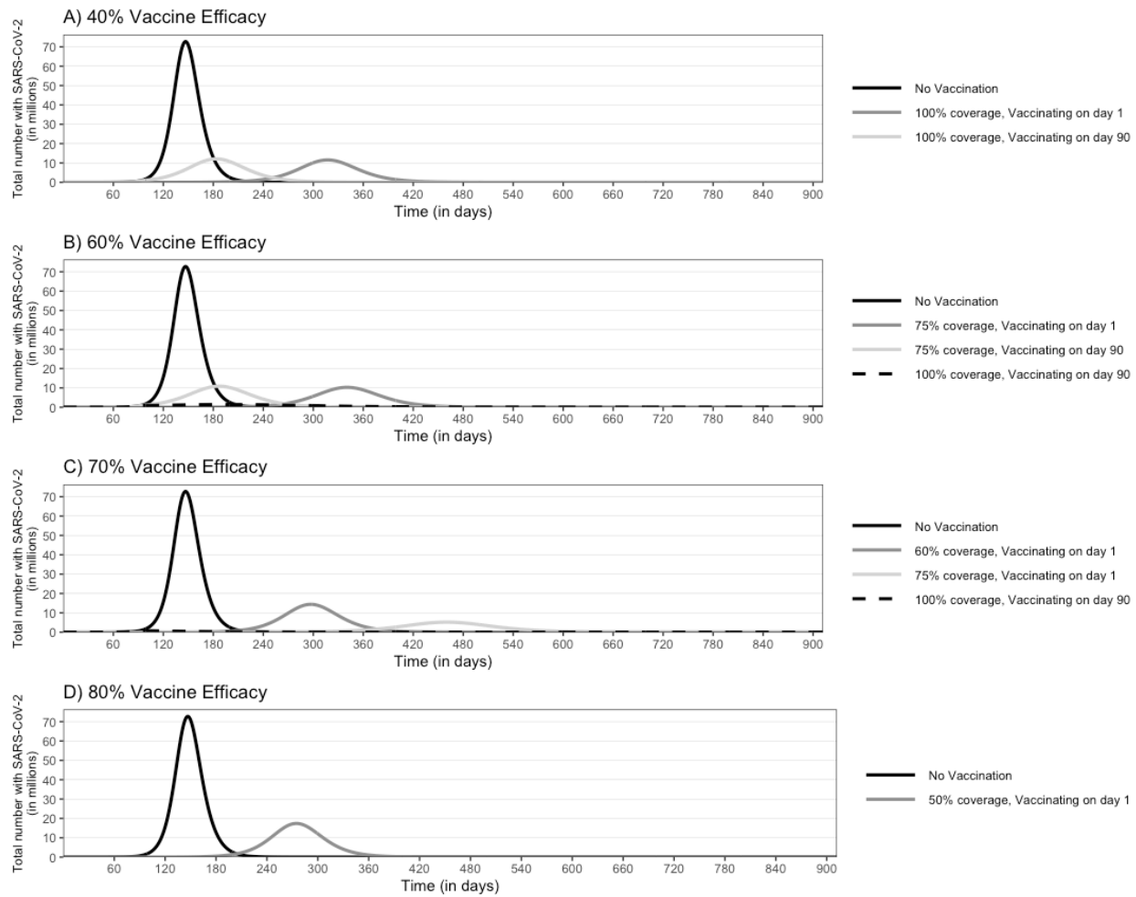
Appendix Figure 1. Epidemic curves for an epidemic with an R_0 of 2.5 and the impact of a vaccine that reduces viral shedding implemented at different points in the epidemic with a vaccine efficacy of A) 40%, B) 60%, C) 70%, and D) 80%
