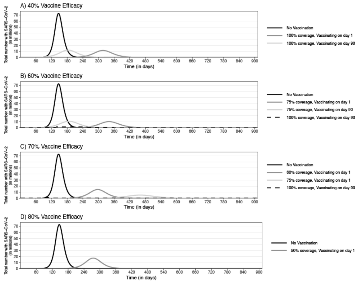
Figure 2. Epidemic curves for an epidemic with an R_0 of 3.5 and the impact of a vaccine that prevents infection implemented at different points in the epidemic with a vaccine efficacy of A) 40%, B) 60%, C) 70%, and D) 80%
