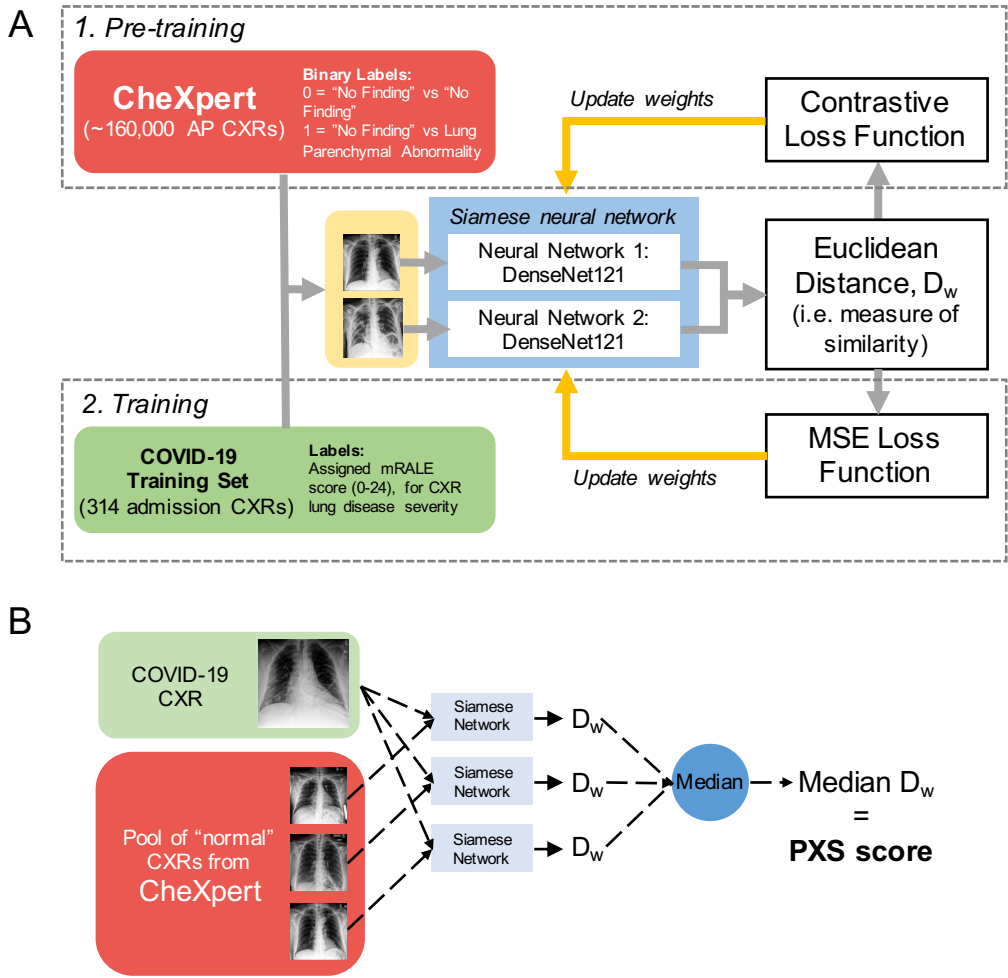
Figure 1: A, Schematic for training the convolutional Siamese neural network-based algorithm used to calculate the Pulmonary X-Ray Severity (PXS) score, a continuous measure of radiographic pulmonary disease severity in COVID-19 patients. The network is pre-trained with chest radiographs (CXRs) from CheXpert (9) using binary lung disease presence labels and then trained on CXRs from a COVID-19 training set using annotations for modified Radiographic Assessment of Lung Edema (mRALE) scores. B, Schematic for calculating the PXS score, which is calculated by comparing the image of interest pairwise with a pool of normal CXRs from CheXpert. D_w = Euclidean distance; MSE loss = mean square error loss.
