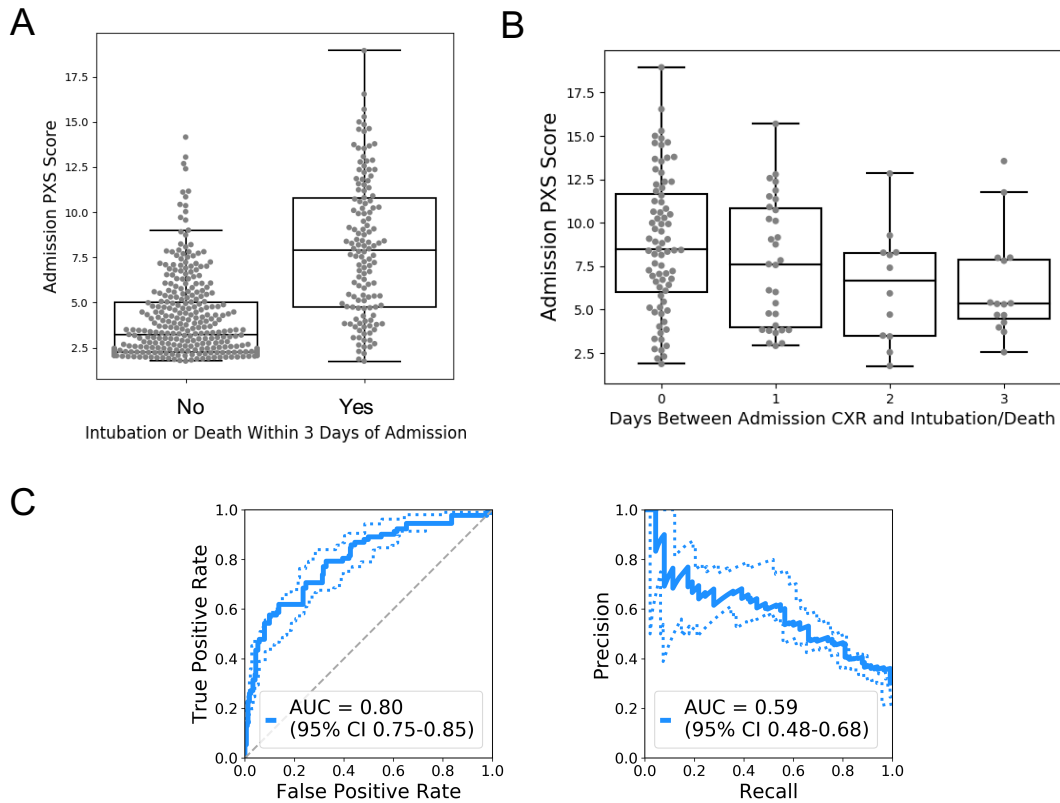
Figure 4: Siamese neural network-based Pulmonary X-Ray Severity (PXS) score is associated with intubation/death in patients hospitalized with COVID-19. A, Boxplot shows the PXS score is significantly higher in patients intubated or dead within three days of hospital admission ( P < 0.001 ). B, Boxplot shows that a higher PXS score is associated with a shorter time interval before intubation or death ( \rho = 0.25 , P = 0.004 ). C, Receiver operator characteristic and precision recall curves show the performance of the PXS score for predicting subsequent intubation or death within three days of hospital admission, in patients without an endotracheal tube on their admission chest radiograph (AUC, area under the curve; dashed lines indicate bootstrap 95% confidence intervals).
