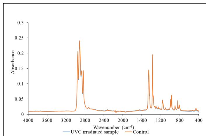
Fig. 3 FTIR spectrum of surgical mask (filtration layer). Orange curve indicates the control sample while blue curve indicates the UVC treated sample at 450 \mu W/cm 2 for 90 minutes.
