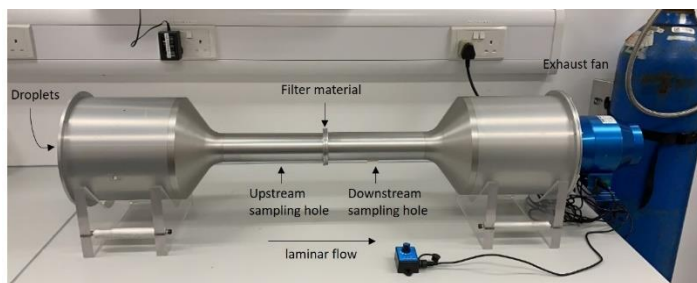
Fig. 1 Setup for filtration efficiency test
