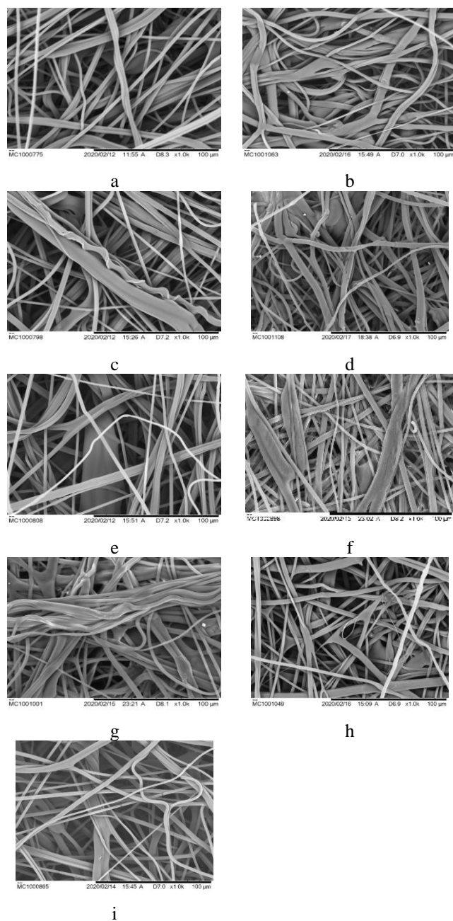
Fig. 2 Appearance of filtration layers of masks after different treatments under scanning electron microscope at 1000 \times . a: control, b: boiled sample, c: steamed sample, d: autoclaved sample, e: detergent treated sample, f: 75% ethanol treated sample, g: 95% ethanol treated sample, h: dry heat sample, i: UVC treated sample
