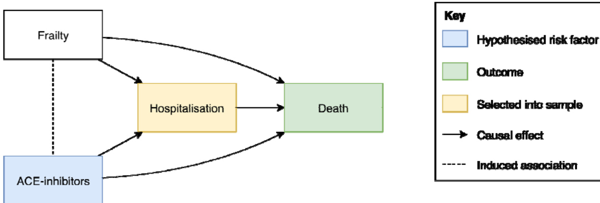
Figure 2: Collider bias induced by conditioning on a collider in three scenarios relating to COVID-19 analysis. These are simplified Directed Acyclic Diagrams where only the main variables of interest have been represented for sake of illustrating collider bias scenarios. All assume no unspecified confounding or other biases. Rectangles represent observed variables and solid directed arrows represent causal effects. The dashed line represents an induced association when conditioning on the collider, which in these scenarios are variables that indicate whether an individual is selected into the sample. (A) When some hypothesised risk factor (e.g. age) and outcome (e.g. COVID-19 infection) each associate with sample selection (e.g. voluntary data collection via mobile-phone apps), the hypothesised risk factor and outcome will be associated within the sample. The presence and direction of these biases are model dependent; where causes are supra-multiplicative they will be positively associated in the sample; where they are sub-multiplicative they will be negatively correlated; and where they are exactly multiplicative they will remain unassociated. We extend this scenario in (B) where the association between the hypothesised risk factor and the collider does not need to be causal.
