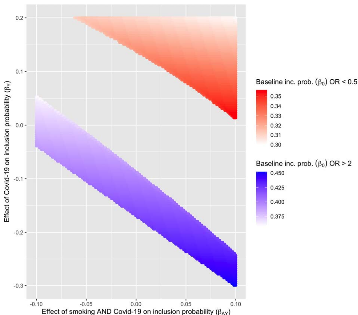
Figure 3: Large associations can be induced by collider bias under the null hypothesis of no causal relationship, using scenarios similar to those reported for the observed protective association of smoking on COVID-19 infection.
