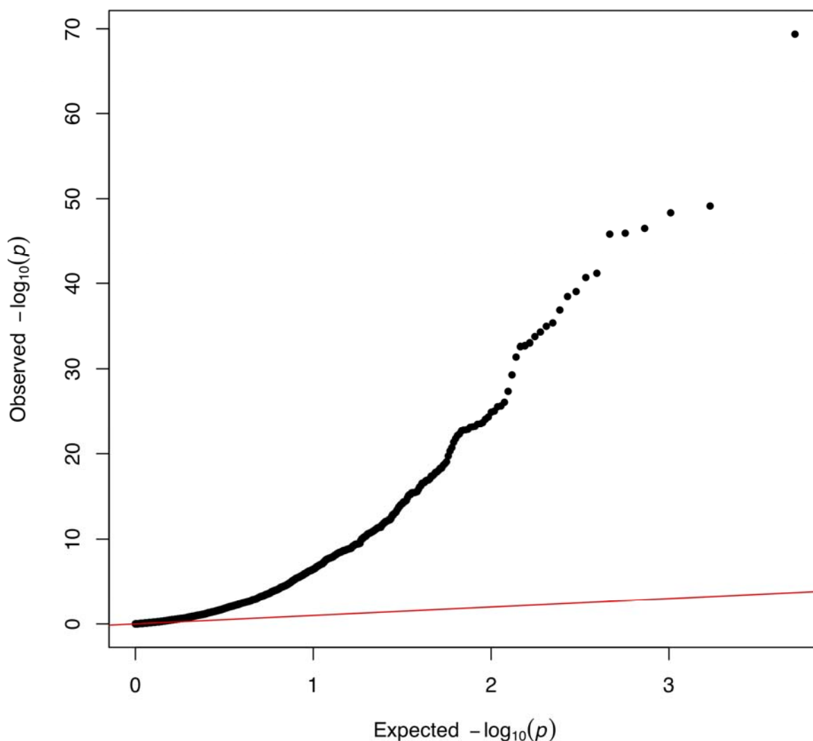
Figure 3: Quantile-Quantile plot of -\log_{10} p-values for factors influencing being tested for COVID-19 in UK Biobank. The x-axis represents the expected p-value for 2,556 hypothesis
