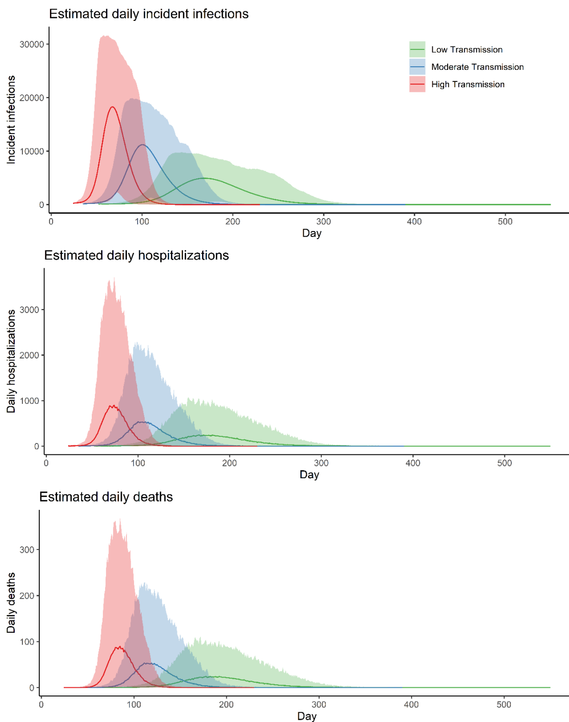
Fig 1. Simulated outbreak trajectories for Kutupalong-Balukhali Expansion Site camps under three transmission scenarios: low transmission ( R_0=1.5-2.0 ), moderate transmission ( R_0=2.0-3.0 ), and high transmission ( R_0=3.3-5.0 ). (A) daily incident number of people infected by COVID-19, (B) daily incident hospitalizations, and (C) daily deaths under the three scenarios. The solid lines represent the mean outbreak trajectories and the shading represents the 95% prediction intervals of each scenario.
