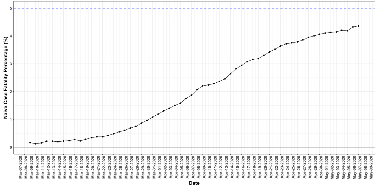
Figure 1. Reported nCFR(t) increases with time after outbreak for Germany. The nCFR has continuously increased with time after the outbreak from a lowest value of 0.12% on March 10, 2020 to its present value on May 7, 2020 of 4.36%. The dashed horizontal line at 5.0% is our estimate of the final CFR from the closed case CFR value.
