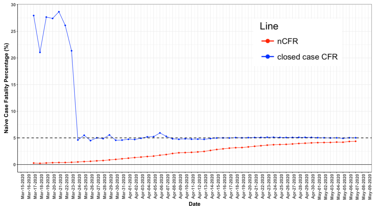
Figure 4. Closed case CFR(t) and nCFR(t) versus day for Germany. As shown by the top curve the closed case fatality ratio appears to be converging to a near constant value. In contrast the nCFR continues to climb and as of May 7, 2020, is still well below the closed case CFR.
