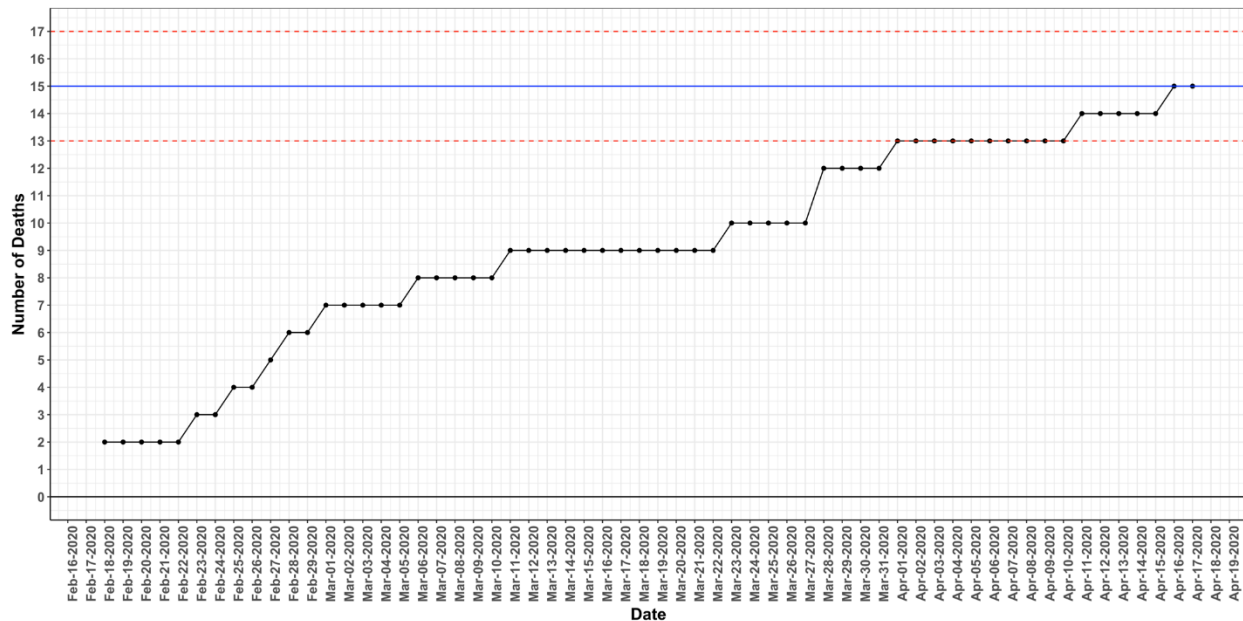
Figure 3. Total number of deaths from February 17, 2020 to April 17, 2020 for the Diamond Princess cruise ship. The solid horizontal line is the number of deaths predicted if the true CFR was 2.1% as predicted by Russell et al. using a similar time to death correction to ours.(6) The red dashed lines are the 95% CI for the estimate. As with the countries examined the number of deaths continues to increase with time.
