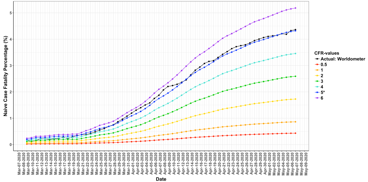
Figure 5B. Simulated and reported nCFR(t) versus day curves for Germany. The reported nCFR(t) curve is plotted in black. Even though the reported nCFR(t) curve rises continuously it is well matched throughout the duration by the calculated nCFR(t) curve (blue) with the final corrected CFR of 5.0%. This corrected CFR is over 10 fold higher than the reported nCFR values early in the outbreak.
