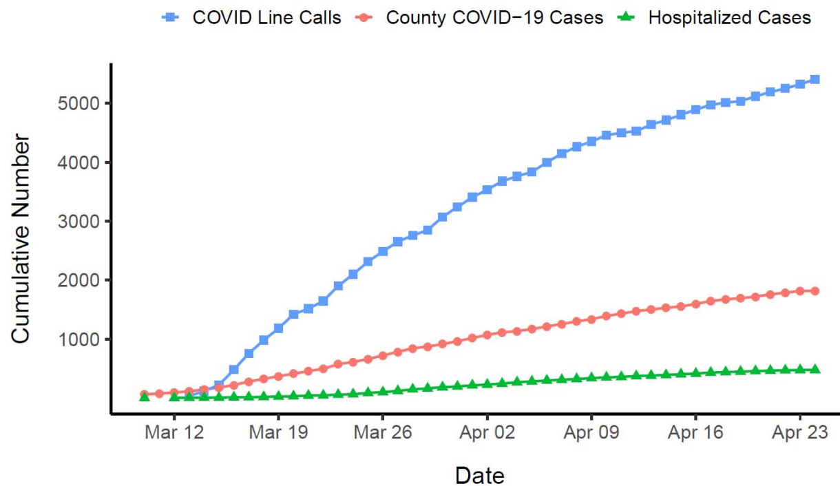
FIGURE 2: COVID-19 Cases (Hotline and Cuyahoga County) and Hospitalizations (County)
